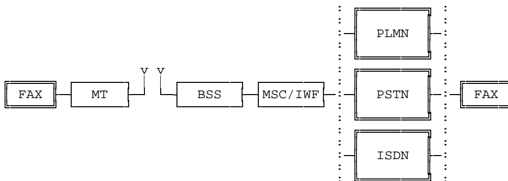
Figure 1/03.46: Network architecture
