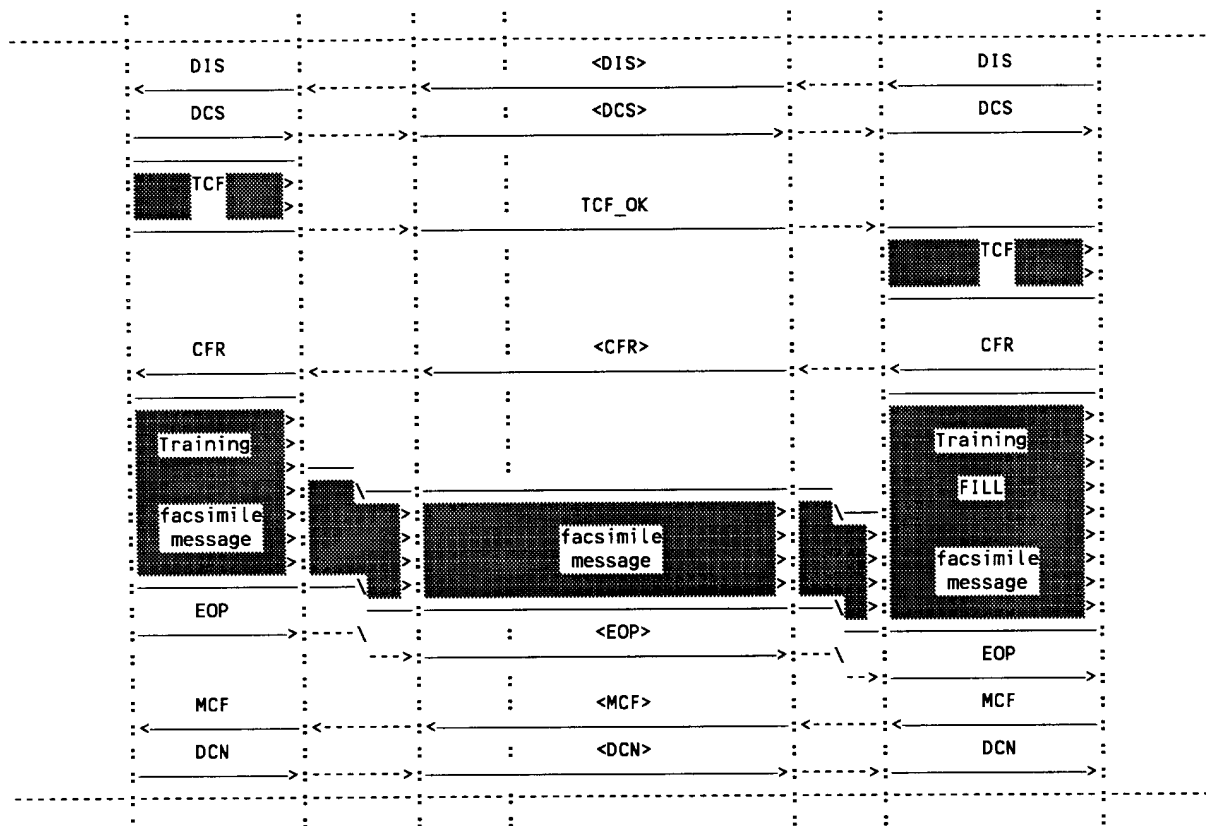
Figure II.6/03.46: Mobile originated facsimile transmission
