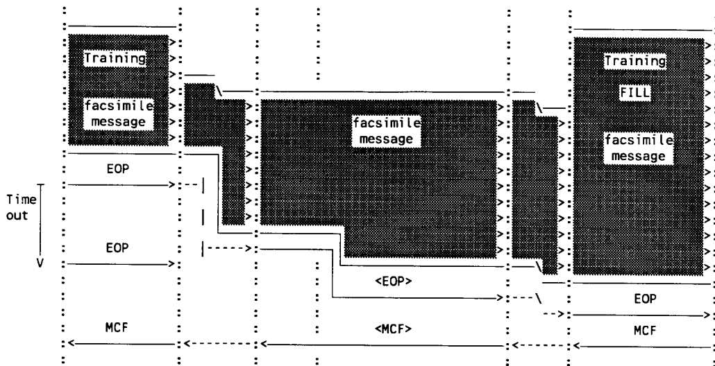
Figure II.13/03.46: Mobile originated facsimile transmission - error recovery (example)
