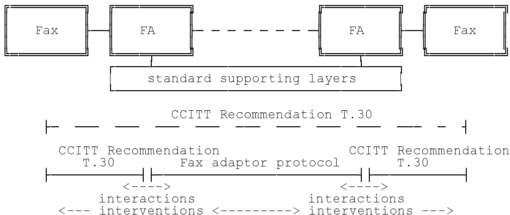
Figure 6/03.46: Communication model
