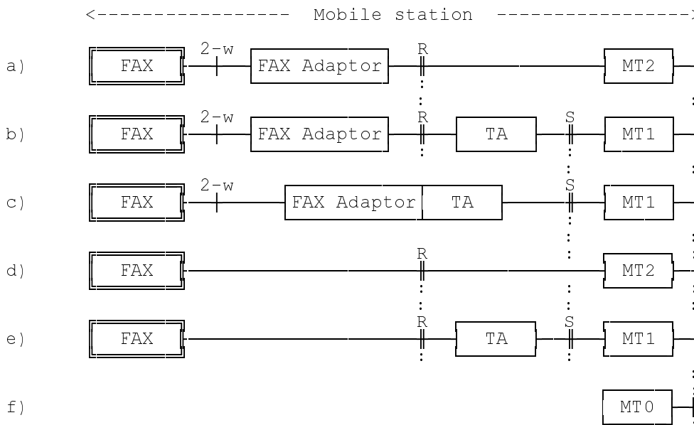
Figure 2/03.46: Reference configurations
