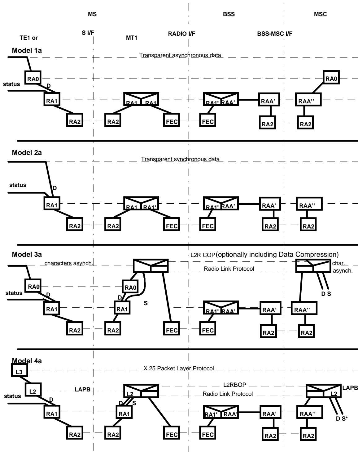
Figure 7: Information transfer protocol models for GSM PLMN connections using 14.4 channels
