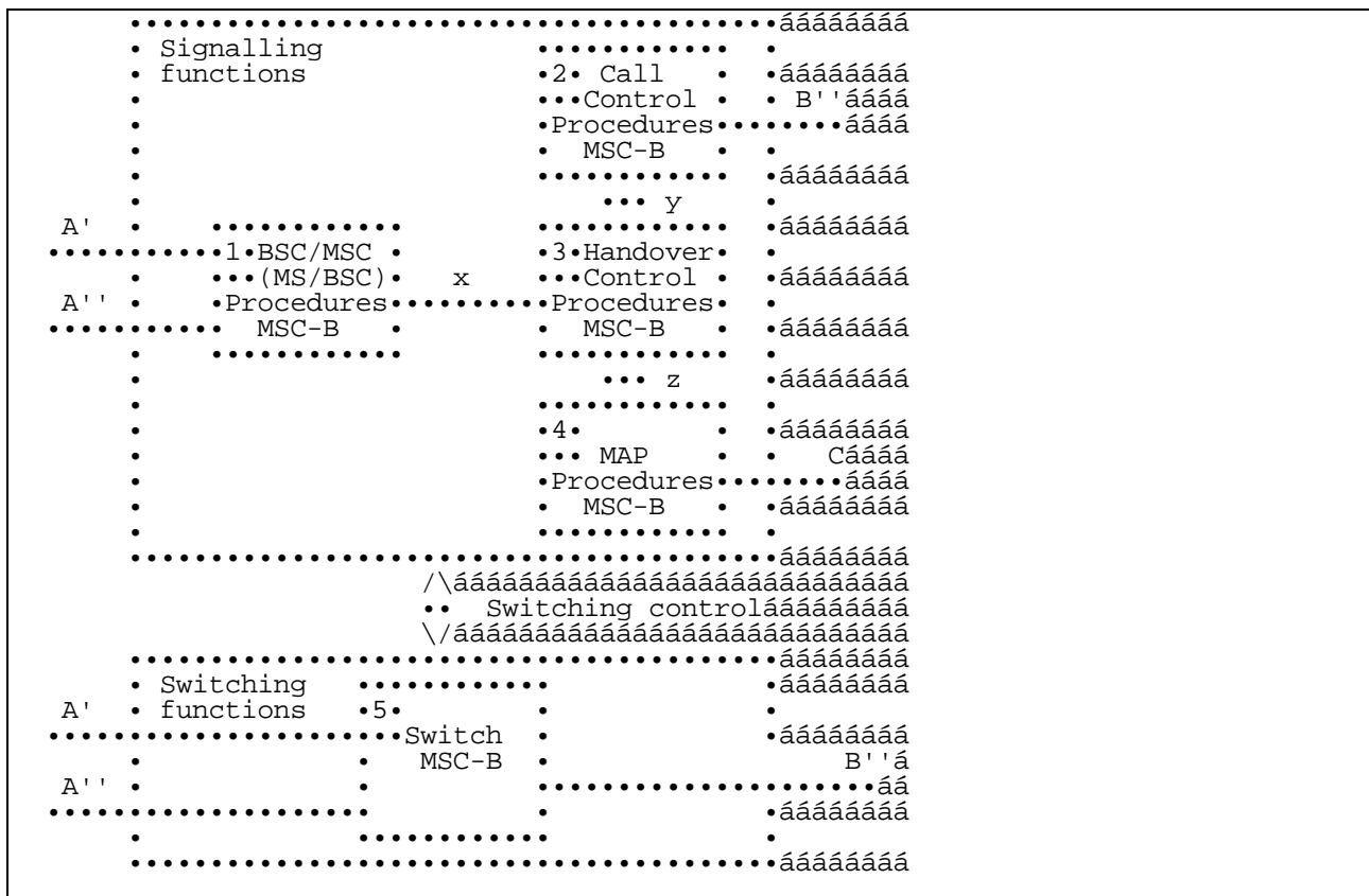
Figure 3: Functional composition of MSC-B for supporting handover
