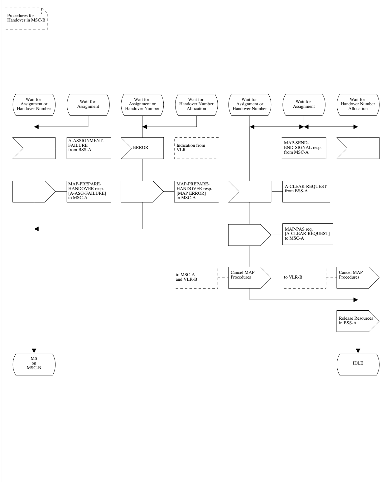
Figure 14 (Sheet 16 of 18): Handover control procedure in MSC-B
