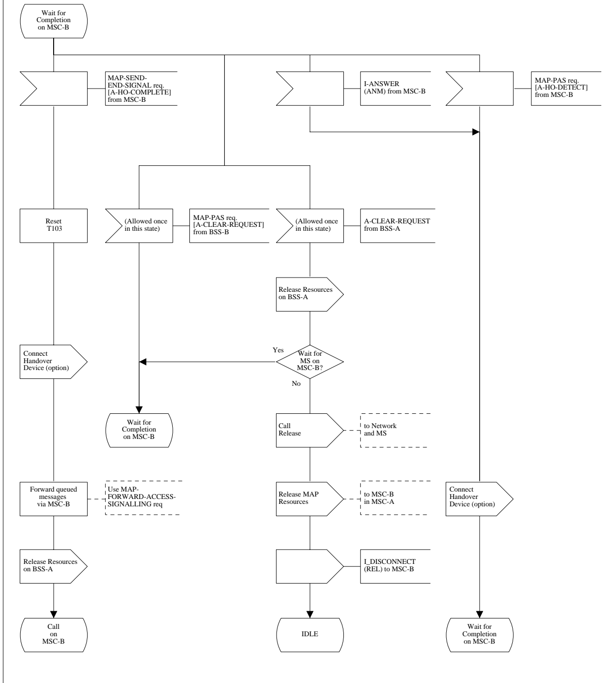
Figure 13 (Sheet 8 of 26): Handover control procedure in MSC-A
