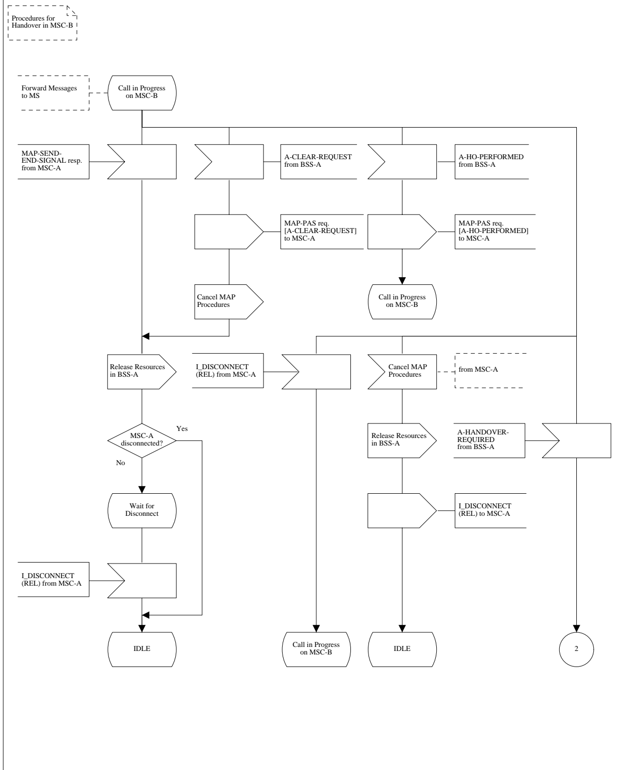
Figure 14 (Sheet 6 of 18): Handover control procedure in MSC-B
