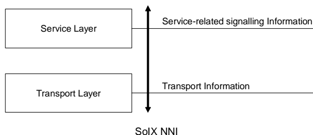
Figure 7a: Solx Interconnection architecture and NNI"
