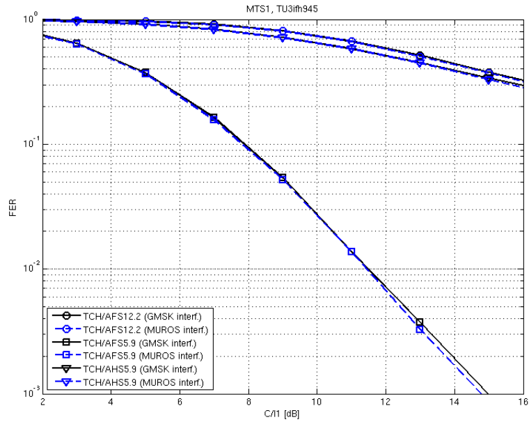
Figure 7-28: DL Co-channel interference performance (MTS1) of a legacy non-DARP MS receiving a MUROS sub channel using AMR half rate 5.9, AMR full rate 12.2 and AMR full rate 5.9
