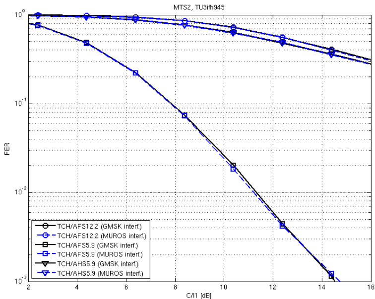
Figure 7-30: DL Mixed interference performance (MTS2) of a legacy non-DARP MS receiving a MUROS sub channel using AMR half rate 5.9, AMR full rate 12.2 and AMR full rate 5.9
