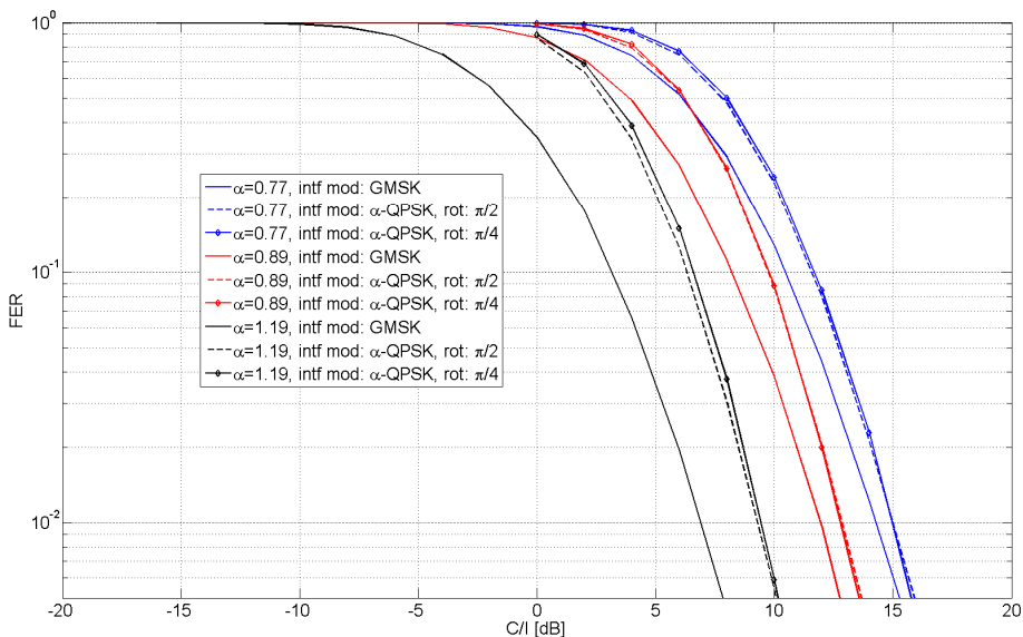
Figure 8-42: SAIC performance when an α-QPSK carrier, using AFS/12.2, is exposed to α-QPSK or GMSK modulated interference
