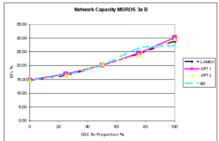
Figure 7-38C2: EFL for investigated TX pulse shapes (MUROS-3a, Channel type B) and different penetrations for OSC aware MS.
