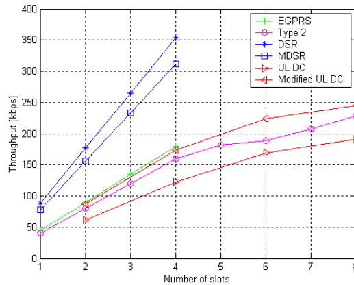
Figure 83: Median throughput (-98 dBm) with multislot profile 3
