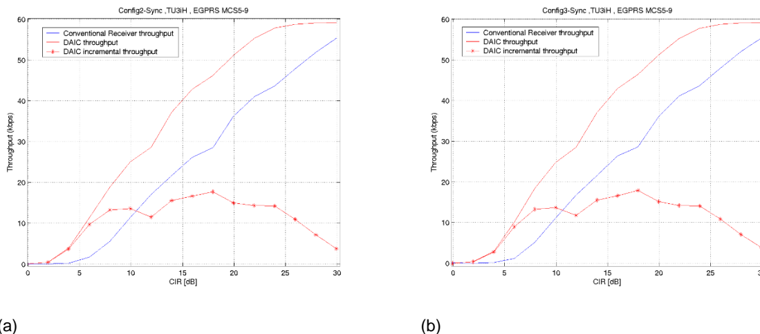
(a) (b) Figure 40: EGPRS Hull-curve comparison of the DAIC and conventional receivers for Synchronized Network (a) Config2 and (b) Config3 [18]
