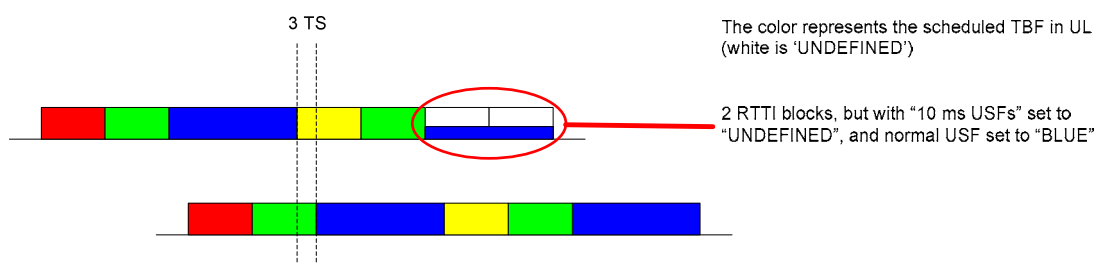
Figure 321: USF scheduling in case of multiplexing with legacy TBFs
