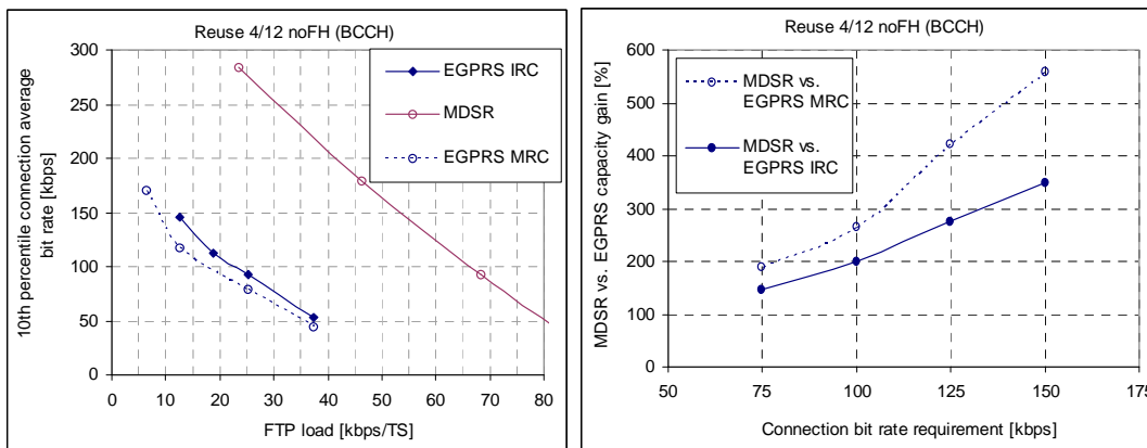
Figure 266: System simulation results for scenario 5 (4/12)
