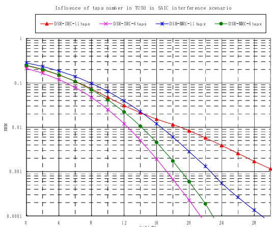
Figure 285: Influence of DSR receiver taps number in TU50 at SAIC interference scenario using two antennas
