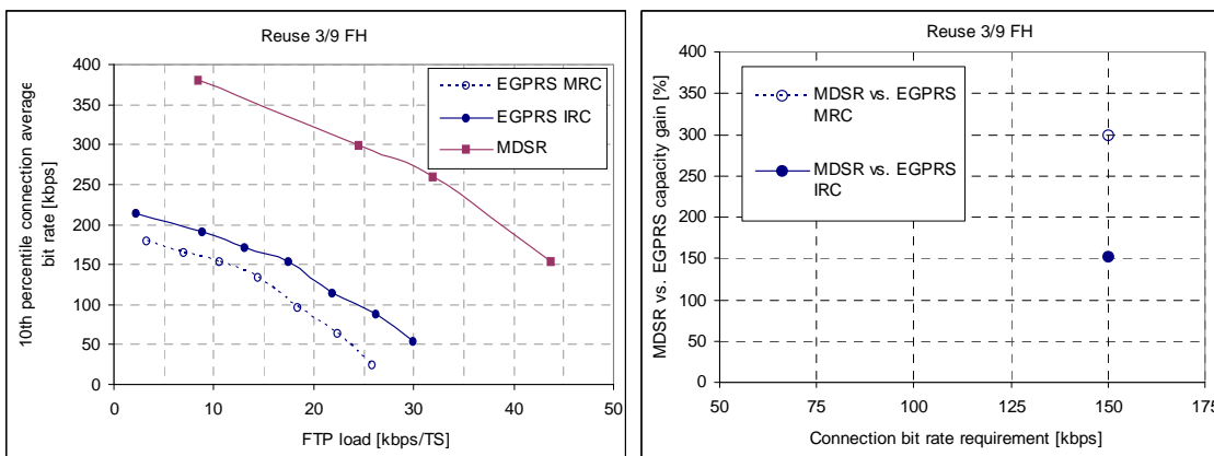
Figure 268: System simulation results for scenario 7 (3/9)
