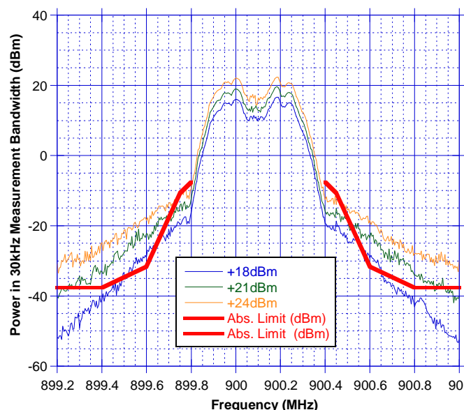
Figure 61: Measured PA output spectrum, dual-carrier input, 200kHz carrier separation.
