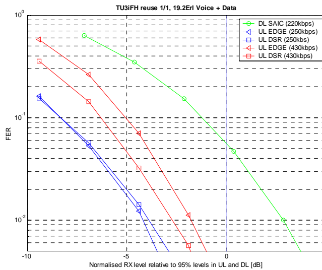
Figure 256: TCH/AFS5.9 FER at re-use 1/1
