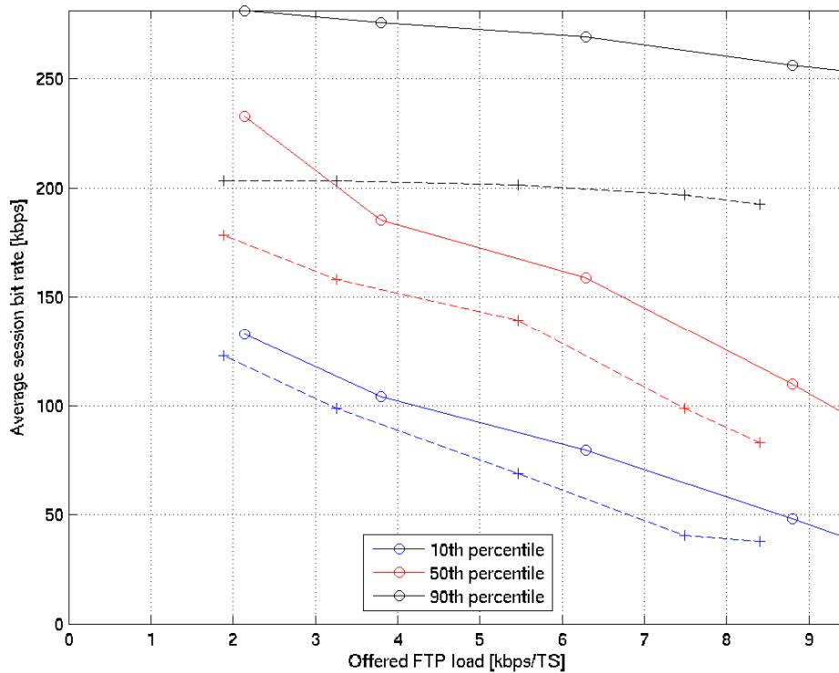
Figure 153b. Average session bit rate percentiles, 10th percentile (blue), 50th percentile (red), 90th percentile (black), as a function of offered FTP load, for EGPRS (dashed) and HQT level 2 (solid), in a 3-reuse.
