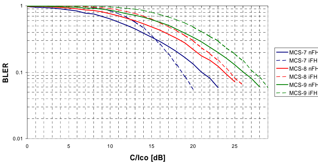
Figure 119: BLER performance for 8-PSK with and without frequency hopping
