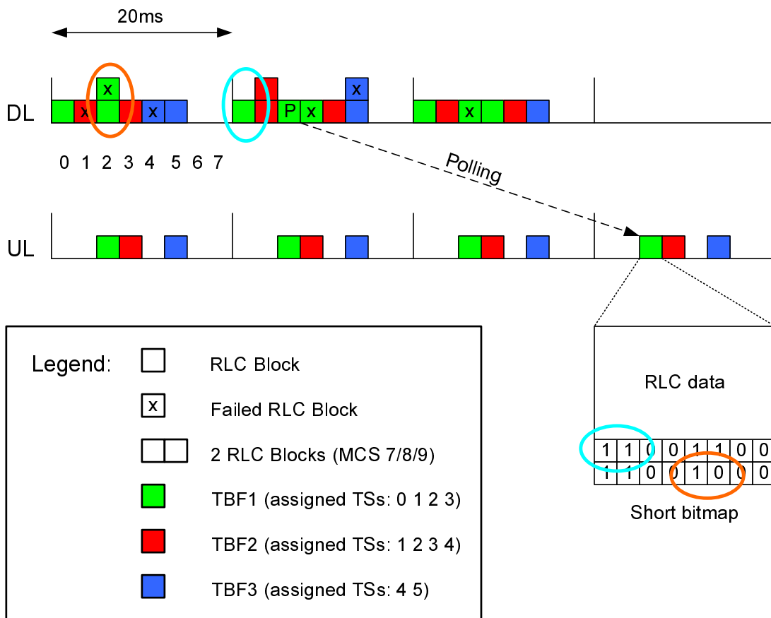
Figure 302: Example of fast ack/nack reporting operation
