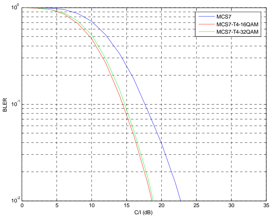
Figure 203: TU3iFH Co-Channel Performance (MCS-7)
