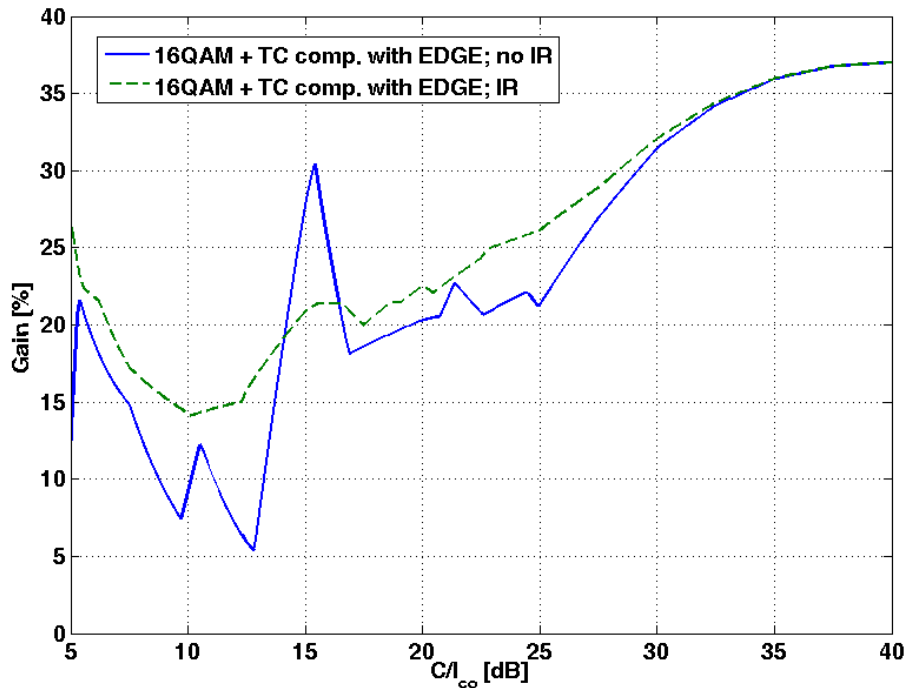
Figure 143: Throughput gain by using HOMTC including MTCS-10 and MCS-11 The different sets are defined in table 53
