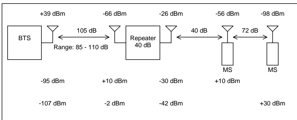
Figure 5: Indoor Repeater Scenario
