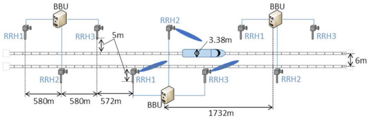
Figure 6.1.5-2: 30 GHz deployment
