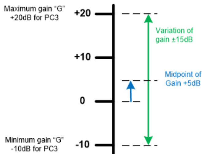
Figure A.2.6.2-1: Example modelling of UE Gain “G” variation
