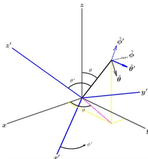
Figure 7.1.3-2: Definition of spherical coordinates and unit vectors in both the GCS and LCS.
