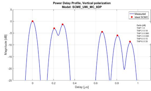
Figure 8.4.2-1a: For MPAC system 1, CE 1 (a) and CE 2 (b) PDP verification measurement for Band 13; for MPAC system 1, CE 1 (c) CE 2 (d) PDP verification measurement for Band 7; For MPAC system 2, PDP verification measurements for Band 13 (e) and Band 7 (f).
