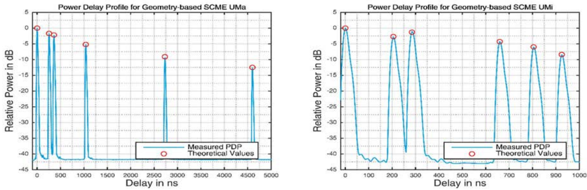
Figure 8.4.2-2a: SCMe UMA and UMi PDP verification measurement for the RTS method with geometric implementation for System 2 with CE2 for Band 13
