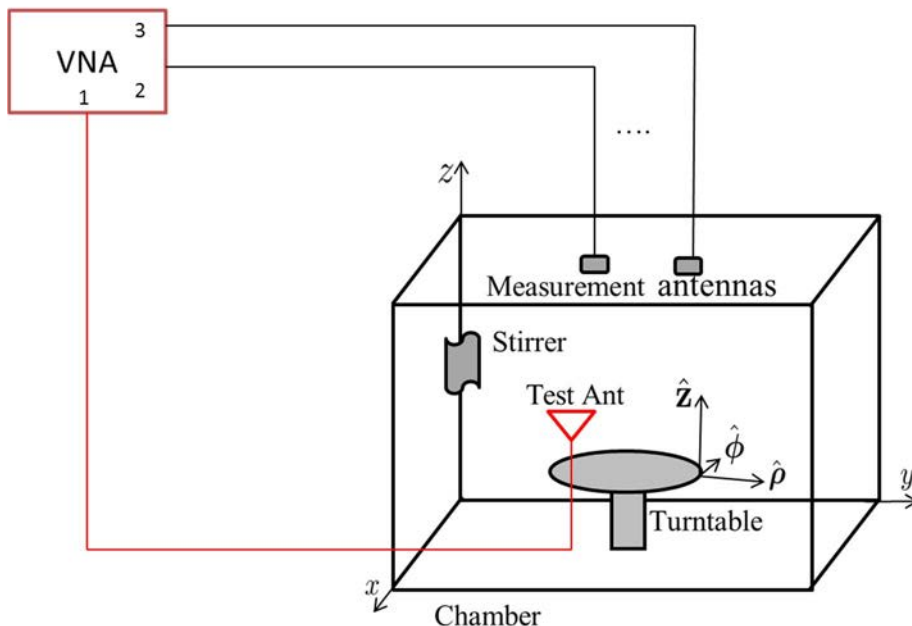
Figure C.3.1.1-2: Setup for VNA measurements for reverberation chamber-only methods
