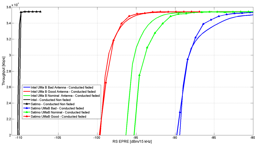
Figure 10.2.2-6: Comparison between the conductive measurements between Intel and SATIMO for the SCME UMaB channel model
