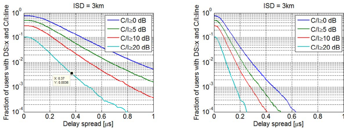
Figure 5.5.4-3: Fraction of users with a certain delay spread and geometry for sub-urban (left) and rural (right)
