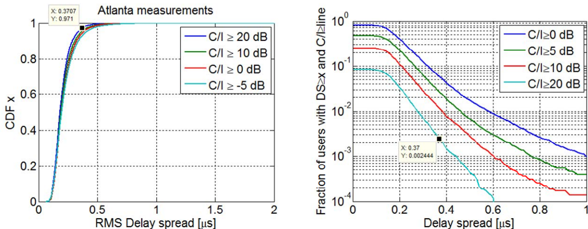
Figure 5.5.4-4: Measured results from Atlanta, GA
