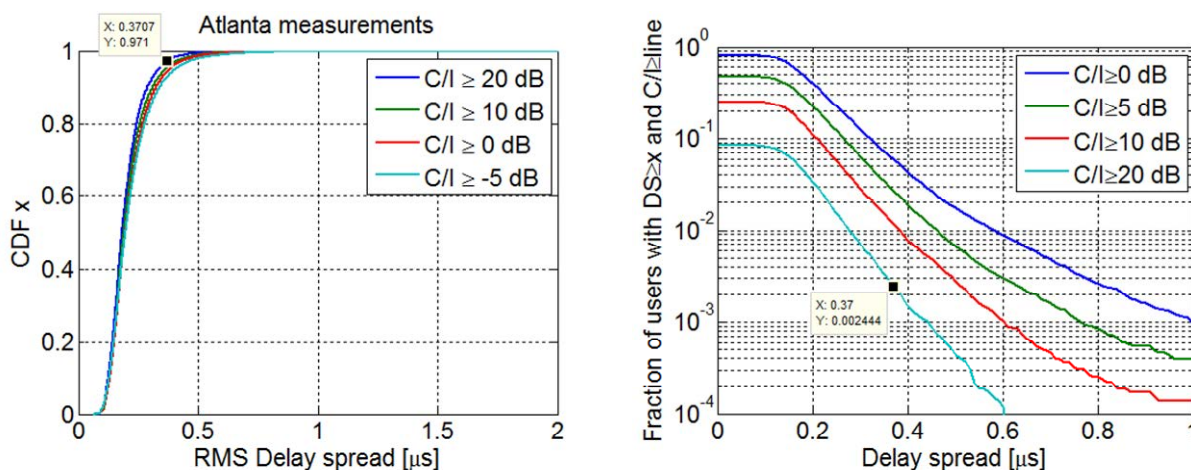
Figure 5.5.4-4: Measured results from Atlanta, GA
