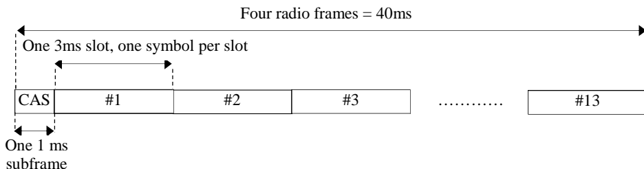
Figure 6.1-2: Frame structure type 1 for transmissions using \Delta f = 0.370 kHz. The CAS is a non-MBSFN subframe, and is configured with 15 kHz subcarrier spacing
