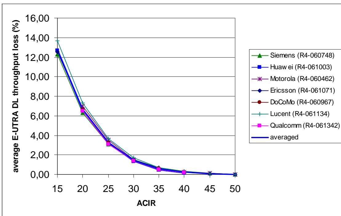
Figure 7.2: average E-UTRA downlink throughput loss
