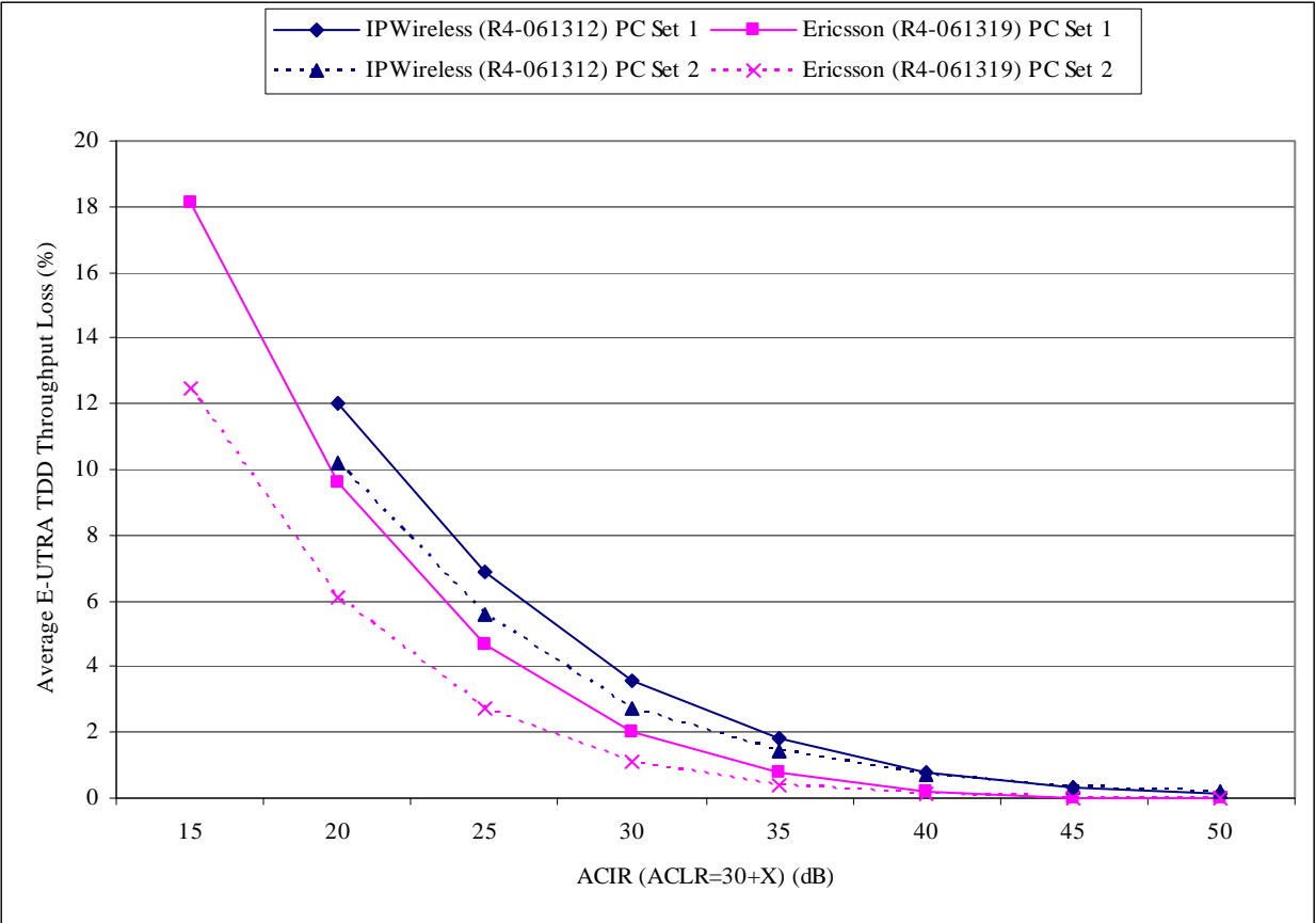
Figure 7.12: average E-UTRA TDD upstream throughput loss
