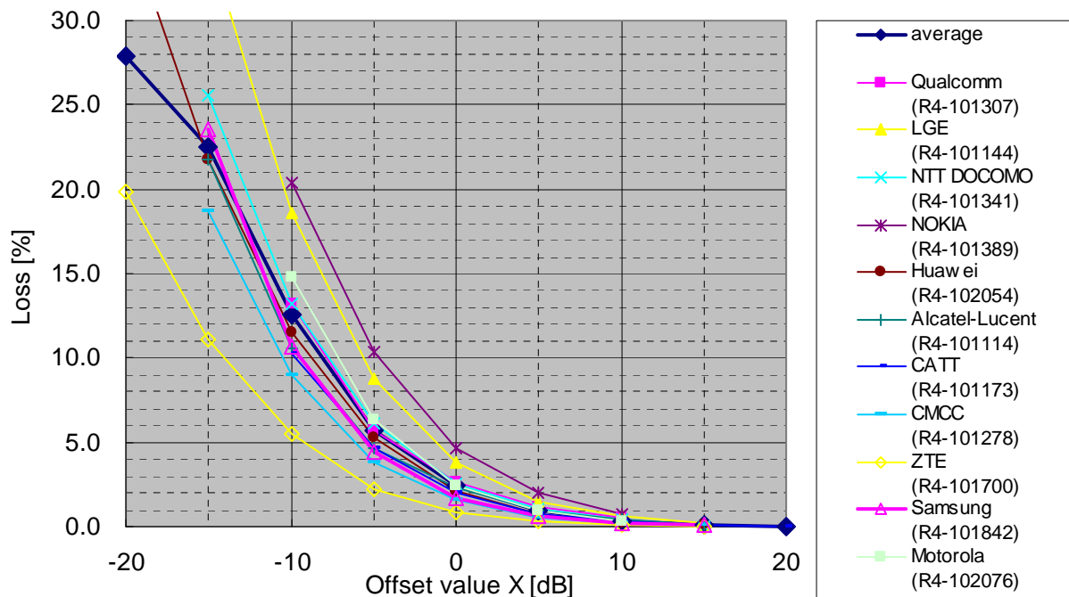
Figure 12.13 average E-UTRA uplink throughput loss (TPC set 1)
