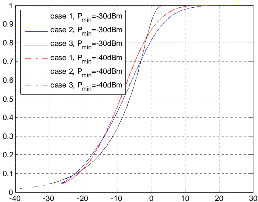
Figure 9.1: LTE UE transmit power CDF (PC set 2)
