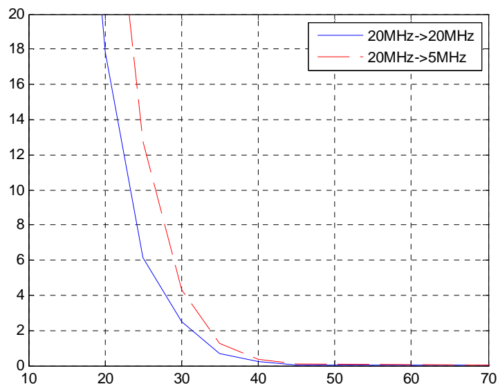
Figure 7.20: Loss in 5%-ile throughput versus ACIR [18]
