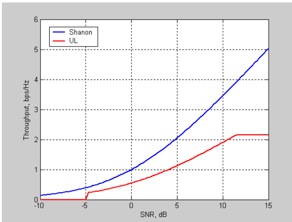
Figure A.7 Throughput vs SNR for Baseline E-UTRA Coexistence Studies for uplink
