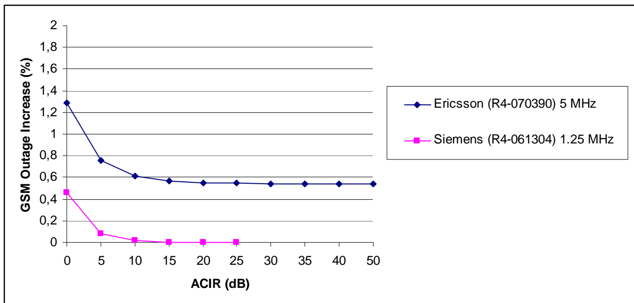
Figure 7.19: GSM uplink outage
