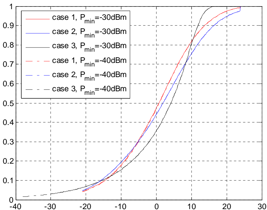
Figure 9.2: LTE UE transmit power CDF (PC set 1)
