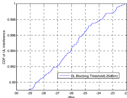
Figure 6.2.4.1-3 CDF of UL interference (Zoom in view)
