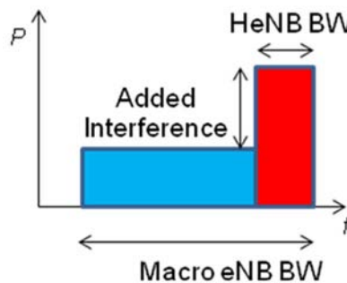
Fig. 7.2.1.2-1 Partial Bandwidth Coexistence
