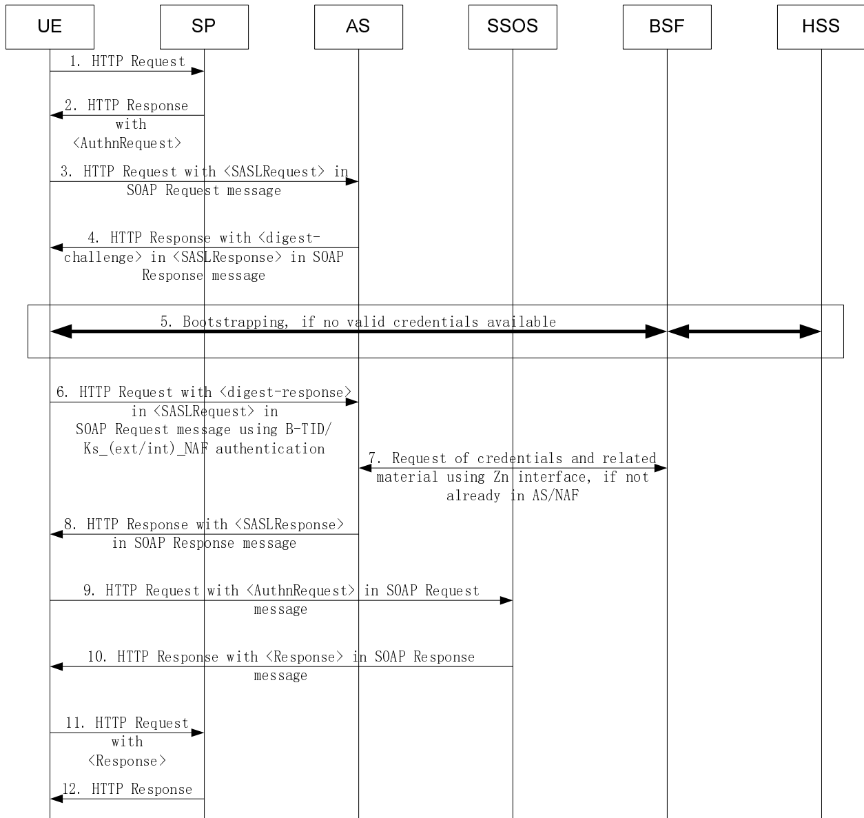
Figure 4.3-3: Message flow for ID-WSF AS and SSOS with Response transfer and usage of GBA
