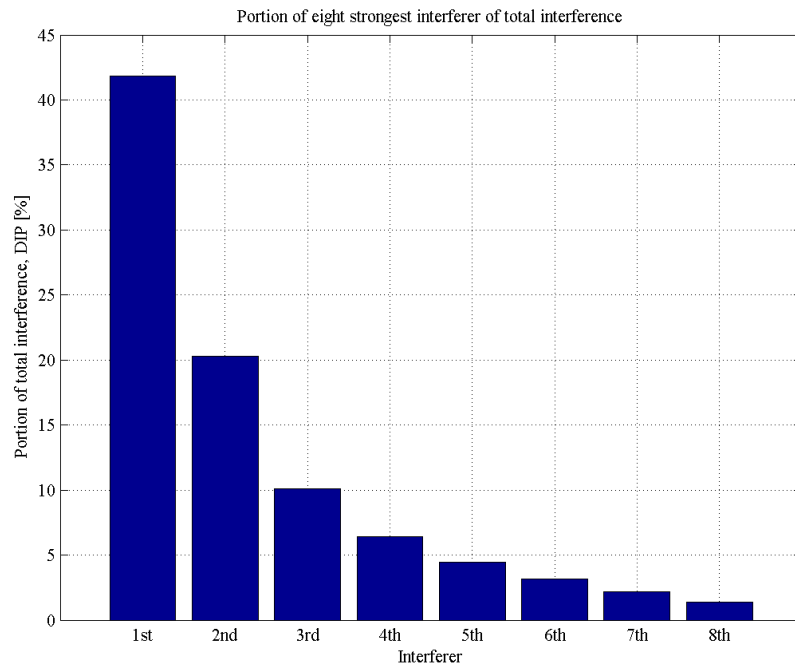
Figure 6.5: 8 Strongest Interferers [9]
