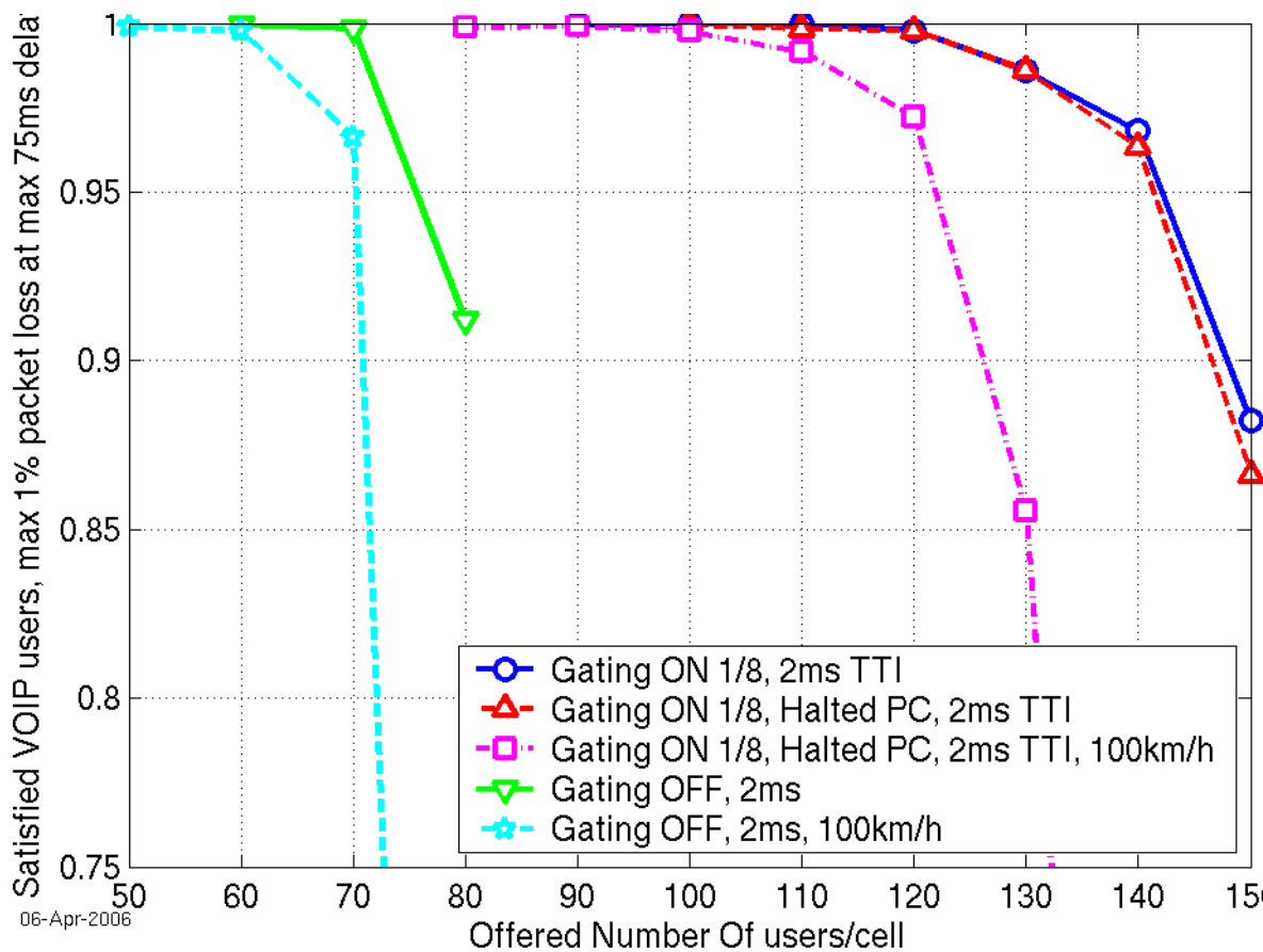
Figure 4.2.2.4.6-1: Capacity gain with gating. HS-DPCCH not modeled.
