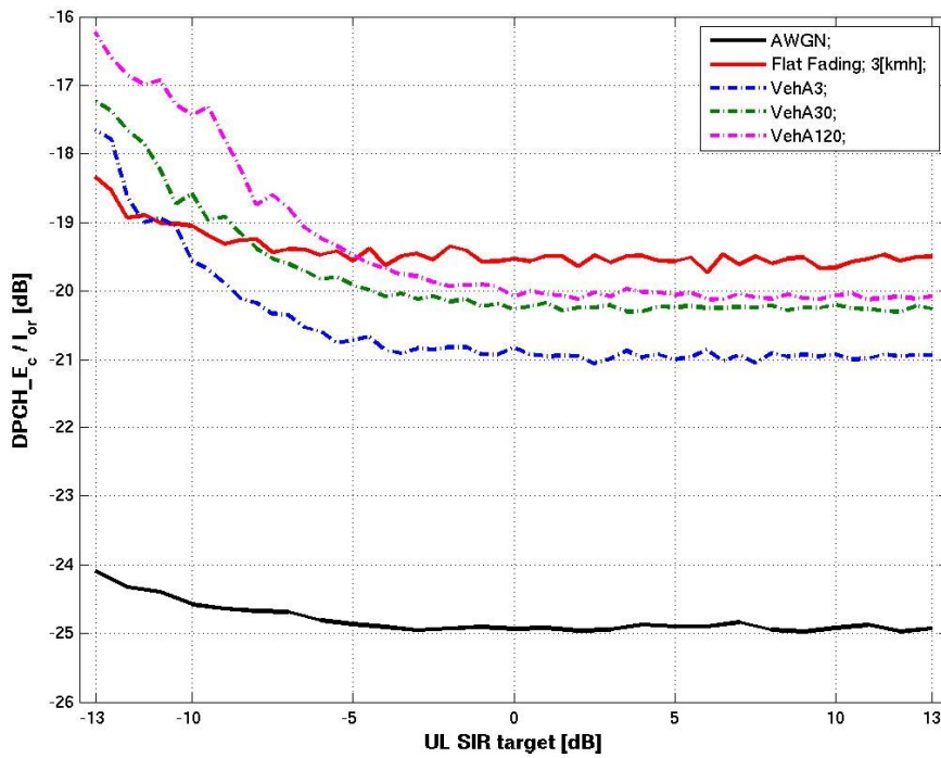
Figure 4.3.2.1.2-1 DL F-DPCH_Ec/I_0R vs. UL DPCCH SIR target
