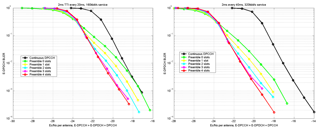
Figure 4.2.2.1-1: BLER vs. Ec/No for different preamble lengths. Vehicular A, 30 km/h
