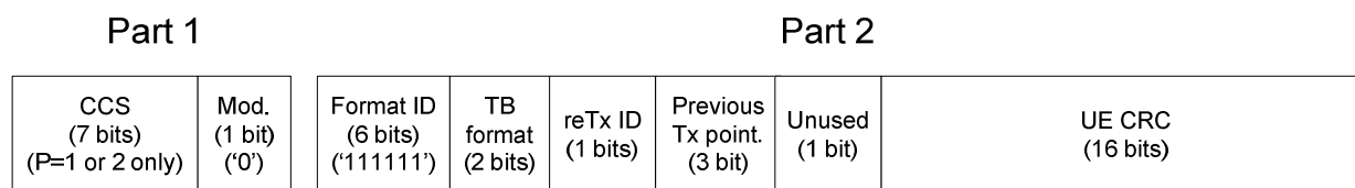
Figure 4.8.1.1-2: Structure of the HS-SCCH for retransmissions using the reduced complexity HS-SCCH-less operation
