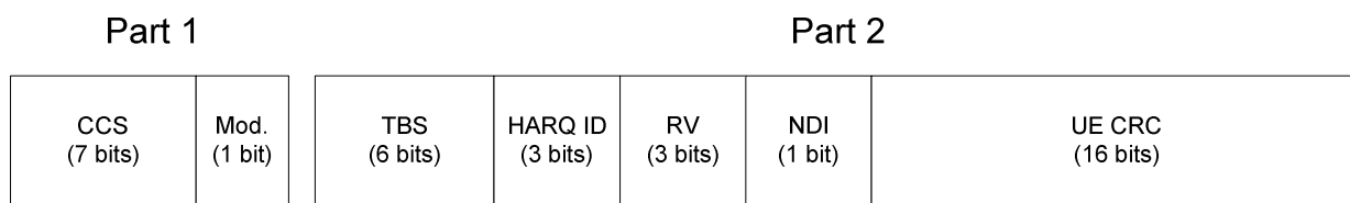
Figure 4.8.1.1-1: Structure of the HS-SCCH for legacy transmissions
