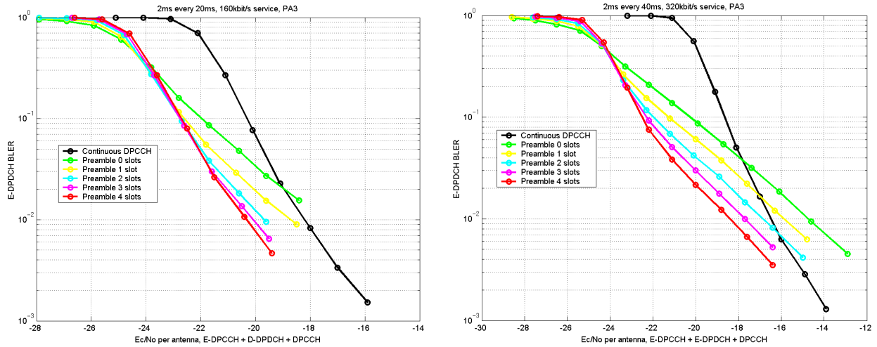
Figure 4.2.2.1-2: BLER vs. Ec/No for different preamble lengths. Pedestrian A, 3 km/h
