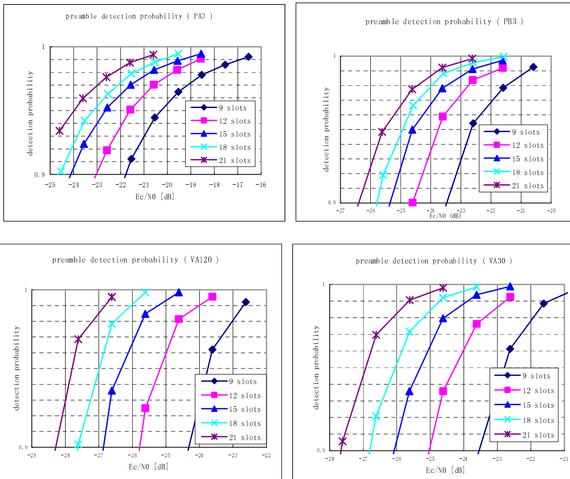
Fig 4.2.2.3.3.2-1. Preamble Detection Probability for different preamble length and various channel models
