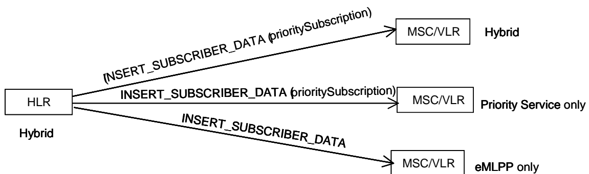
Figure C.2: Hybrid HLR
