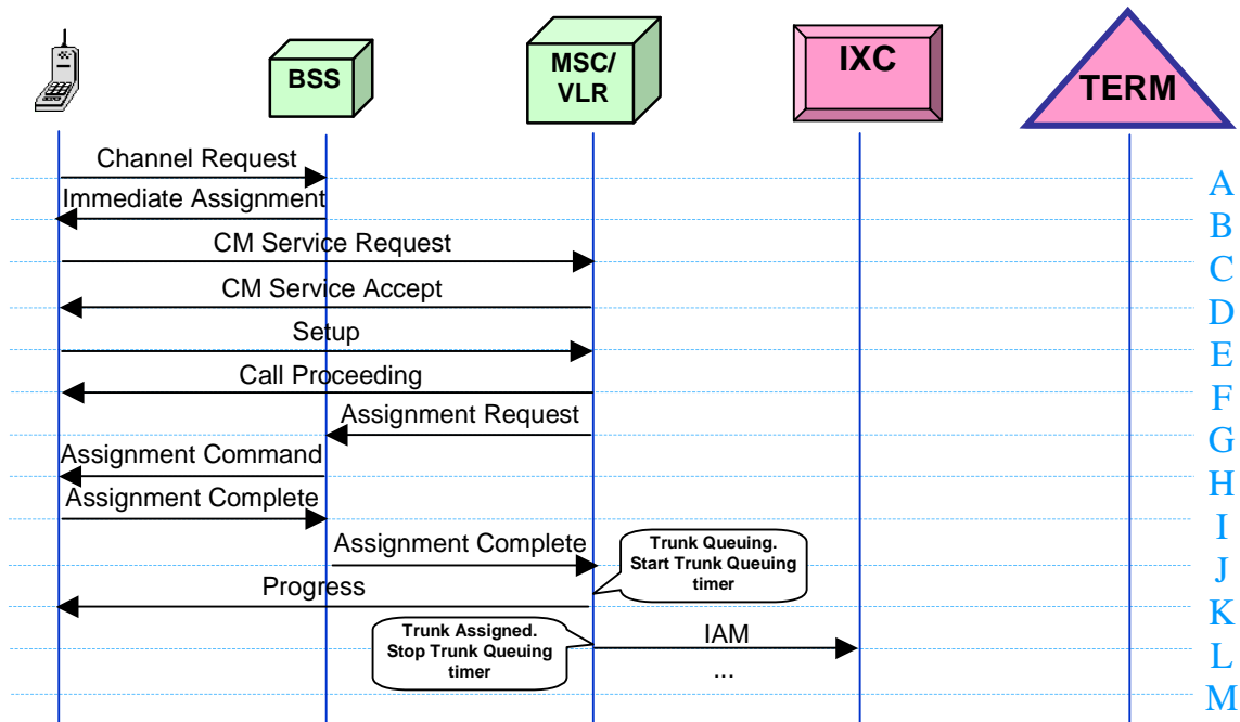
Figure 5.11: Call Progression – MSC – Outgoing Trunk Queuing
