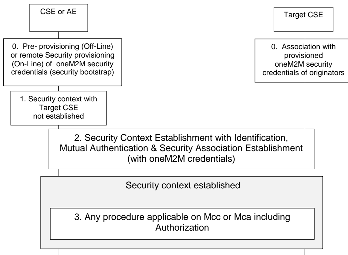
Figure 7: High Level Procedures on Mcc or Mca
