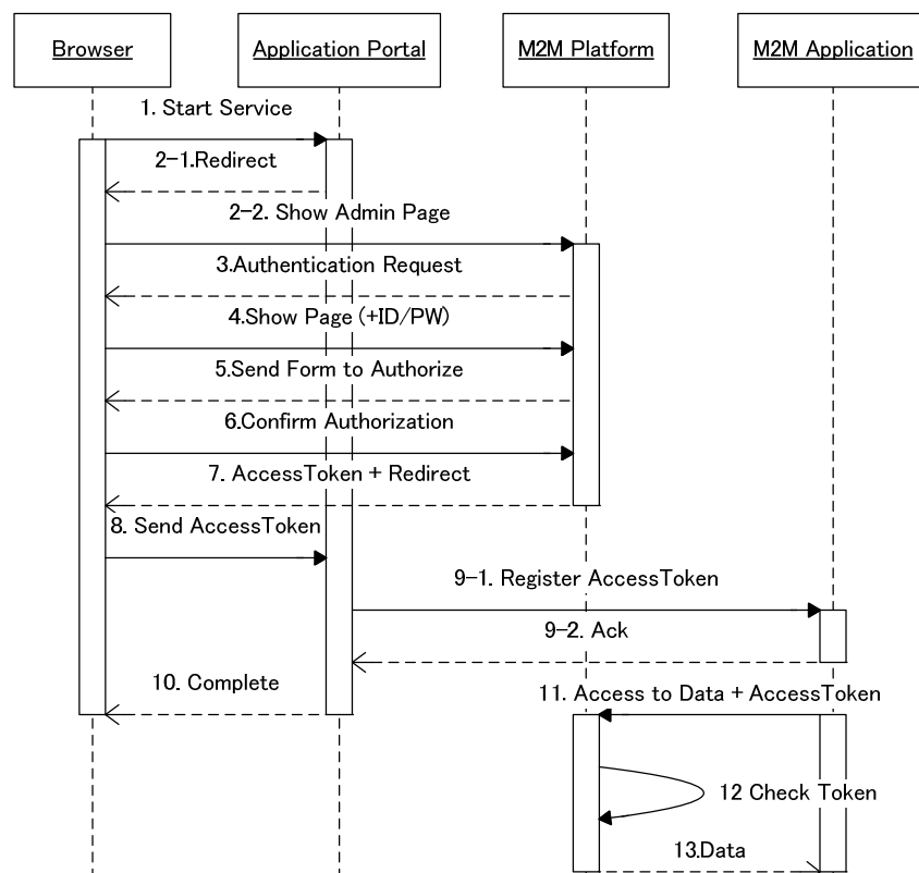
Figure 2: OAUTH flow
