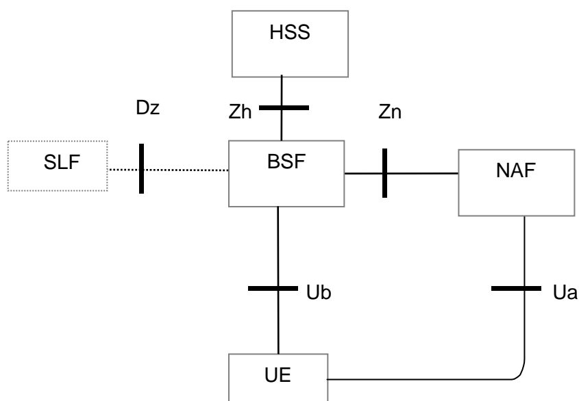
Figure 5a: Simple Network Architecture for GBA in 3GPP [i.8]
