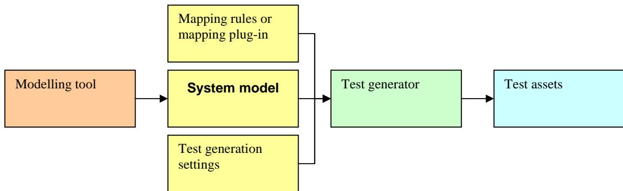
Figure 2: Process for model-based testing with system models
