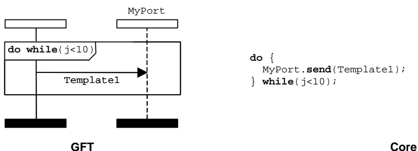
Figure 28: Do-while statement
