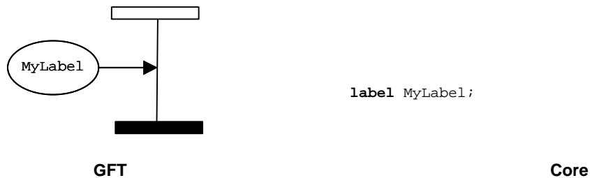
Figure 22: Label statement
