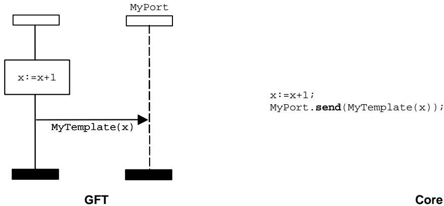
Figure 29: Sequential behaviour
