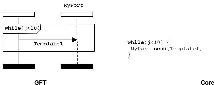
Figure 27: While statement
