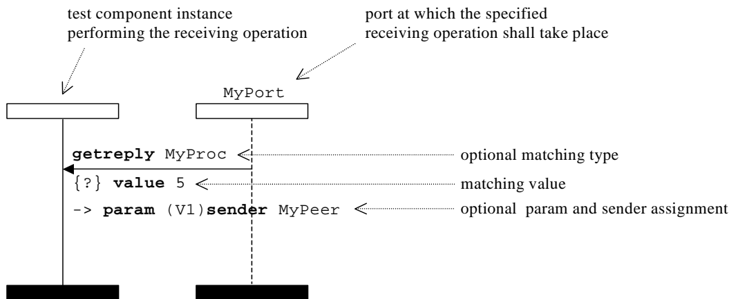
Figure 51: General format of receiving operations with param and sender assignment
