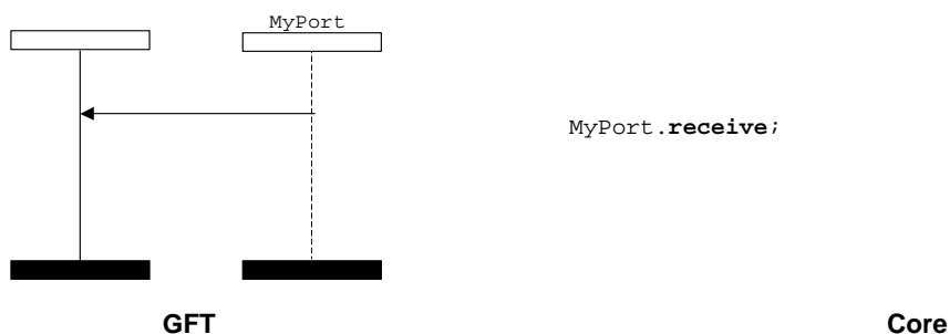
Figure 56: Receive any message
