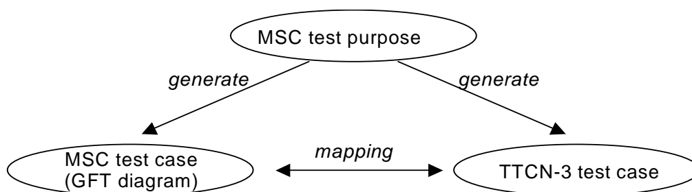
Figure 4: Relations between MSC test purpose description, MSC test case descriptions and TTCN-3
