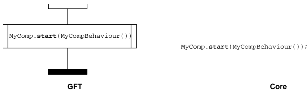
Figure 44: Start operation
