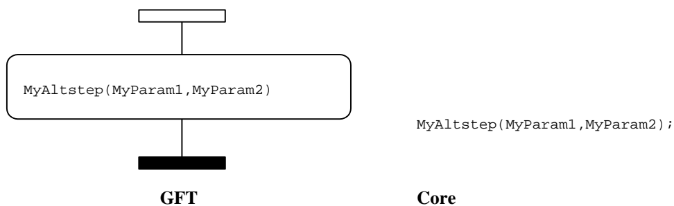
Figure 19: Altstep invocation
