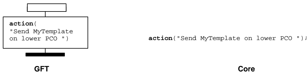
Figure 111: External actions
