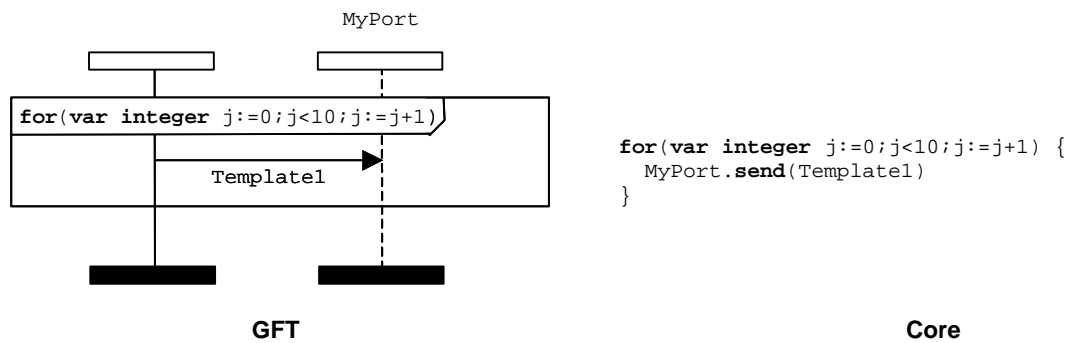
Figure 26: For statement
