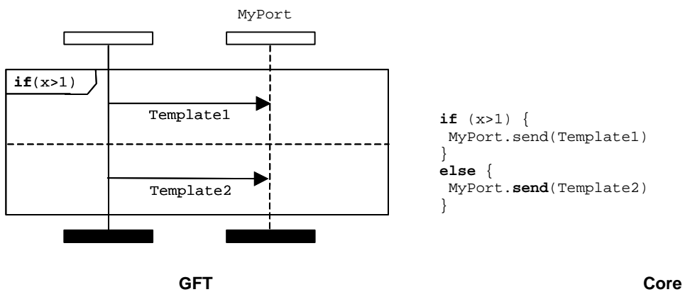
Figure 25: If-else statement
