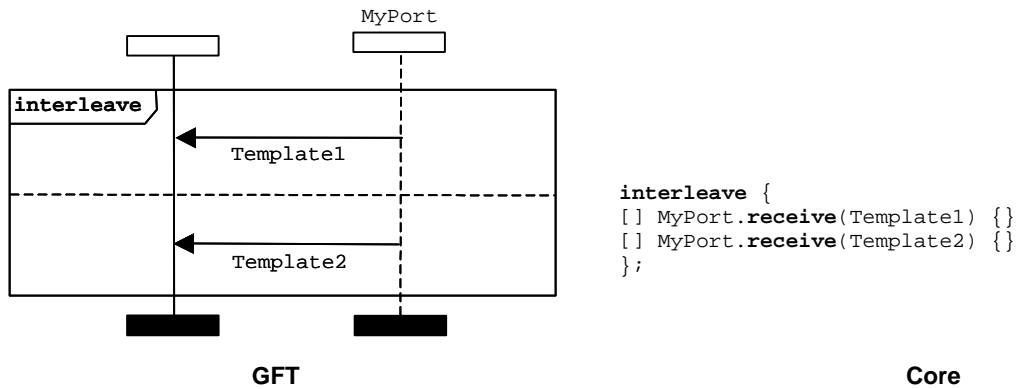
Figure 36: Interleave statement
