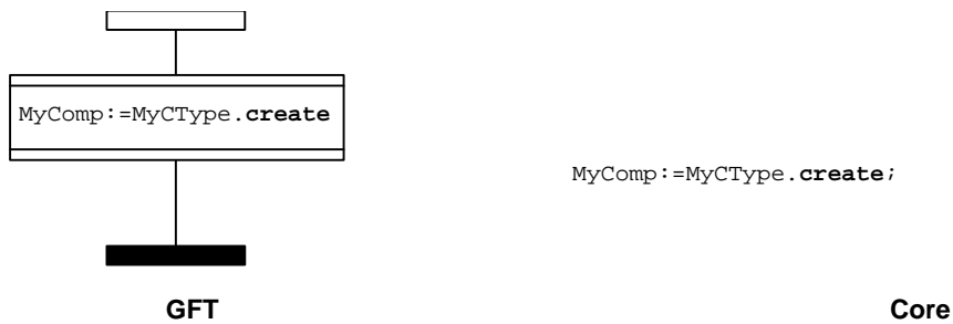
Figure 41: Create operation
