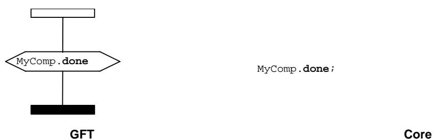
Figure 48: Done operation
