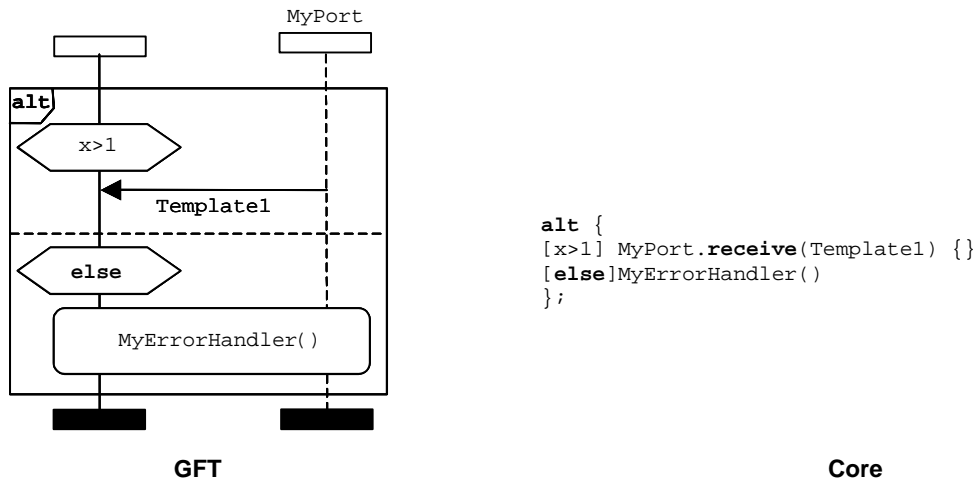
Figure 34: Else within an alternative
