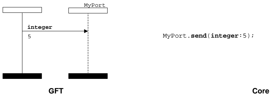
Figure 53: Send operation with inline template
