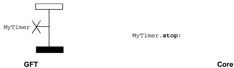
Figure 103: The stop timer operation
