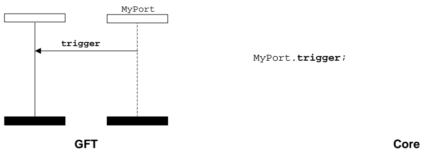
Figure 60: Trigger on any message operation
