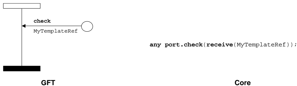
Figure 97: Check a receive on any port
