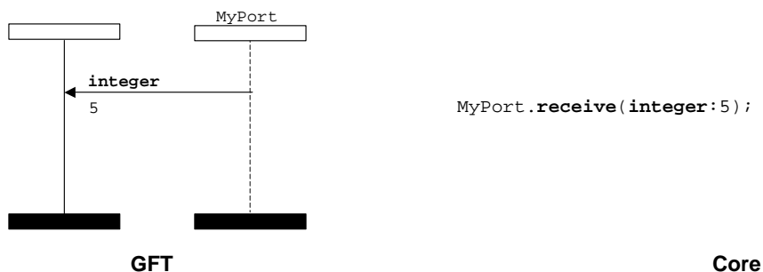
Figure 55: Receive operation with inline template
