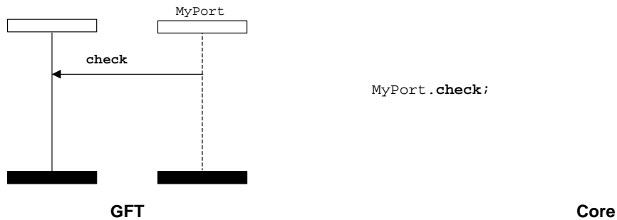
Figure 96: Check any operation
