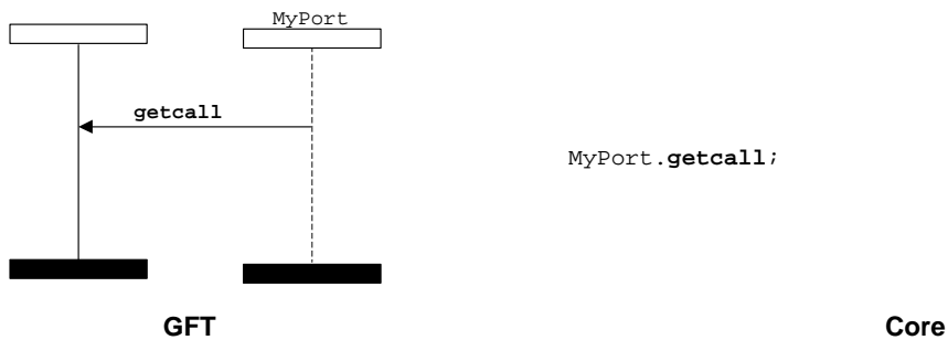
Figure 70: Getcall on any call operation
