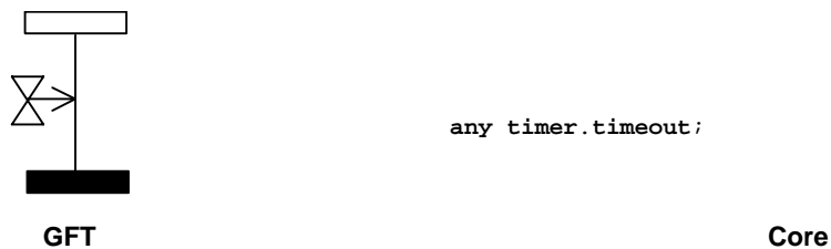
Figure 109: Timeout from any timer
