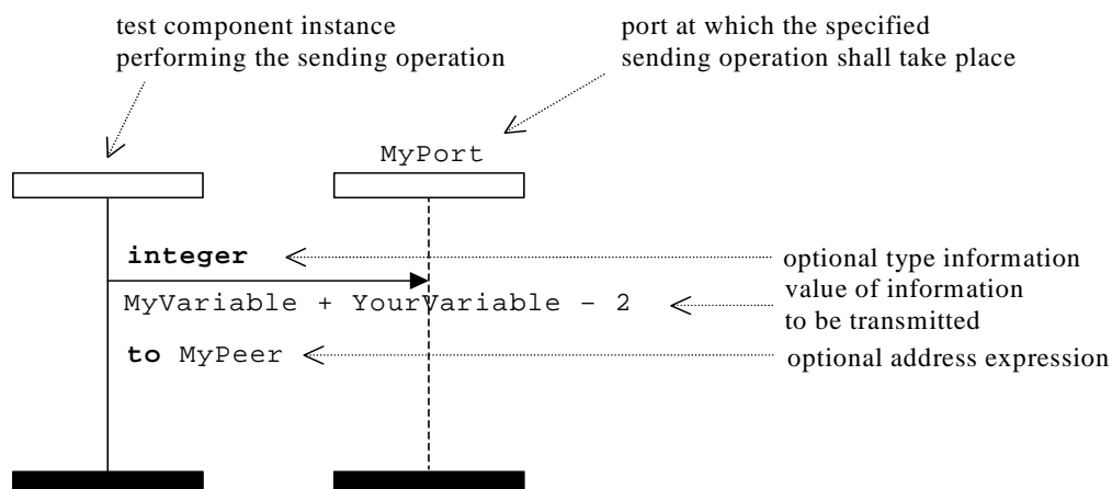
Figure 49: General format of sending operations
