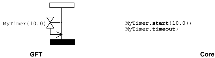
Figure 106: Connected start and timeout timer symbols
