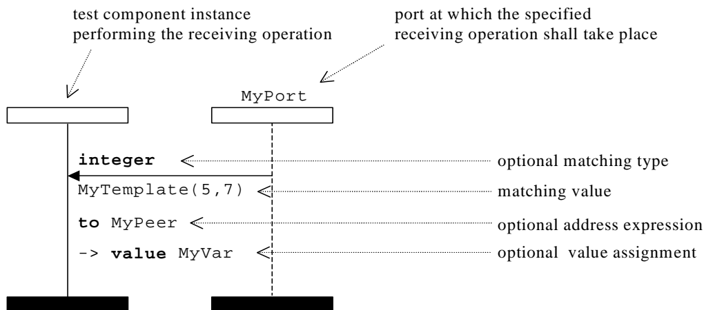
Figure 50: General format of receiving operations with address and value assignment
