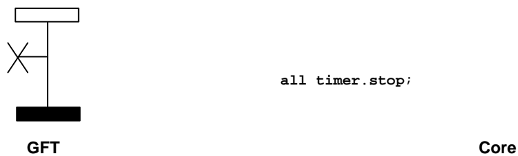
Figure 108: Stopping all timers
