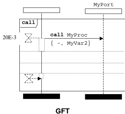
Figure 65: Blocking call operation followed by timeout exception
