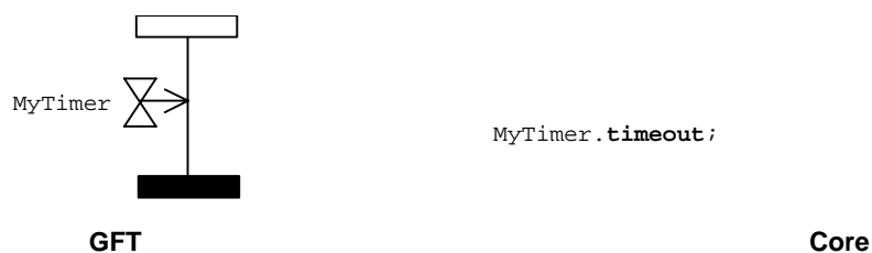
Figure 105: The timeout operation
