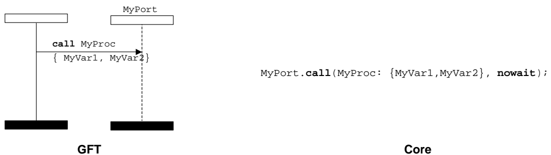
Figure 67: Non-blocking call operation with inline template
