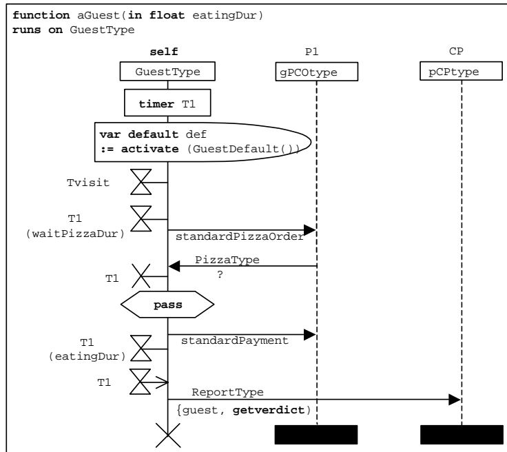
Figure E.2: Restaurant example - newInternetPTC and aGuest functions
