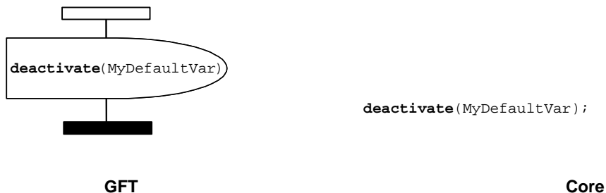
Figure 40: Deactivation of defaults
