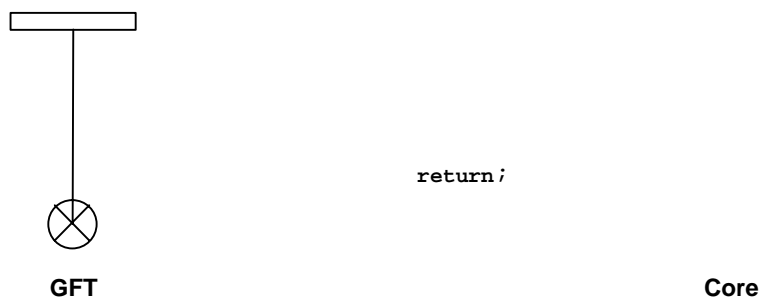
Figure 37: Return symbol without a return value
