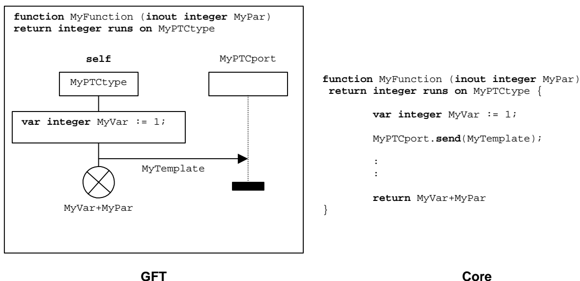
Figure 11: Principle shape of a GFT function diagram and corresponding core notation
