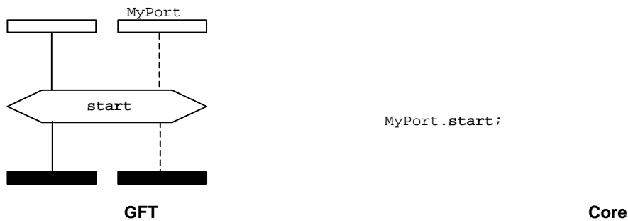
Figure 99: Start port operation
