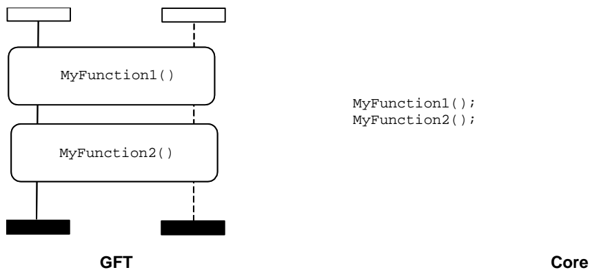
Figure 30: Sequencing using references
