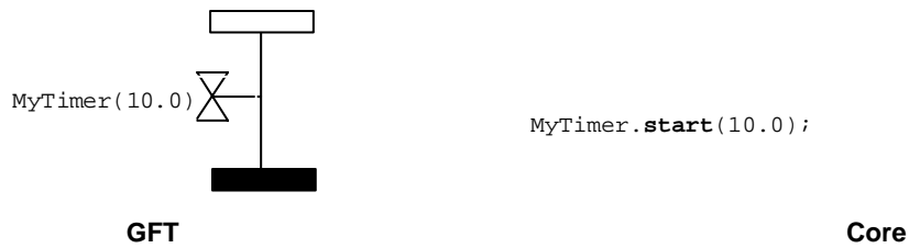
Figure 102: The start timer operation
