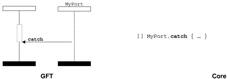
Figure 89: Catch any exception (within a call symbol)
