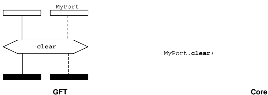
Figure 98: Clear port operation
