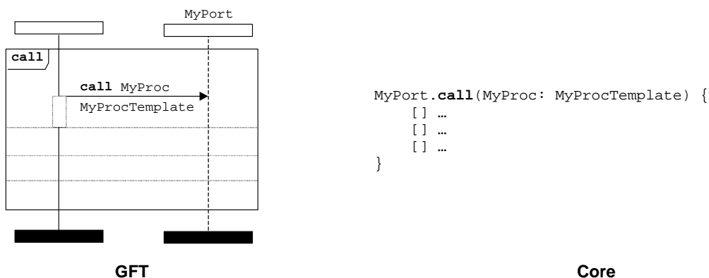
Figure 62: Blocking call operation with template reference
