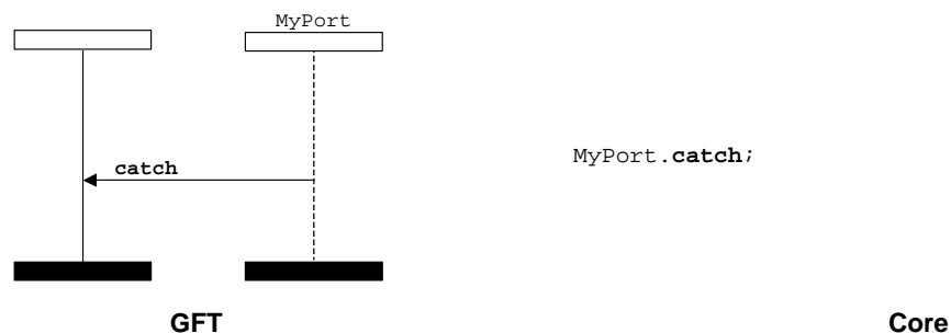
Figure 90: Catch any exception (outside a call symbol)
