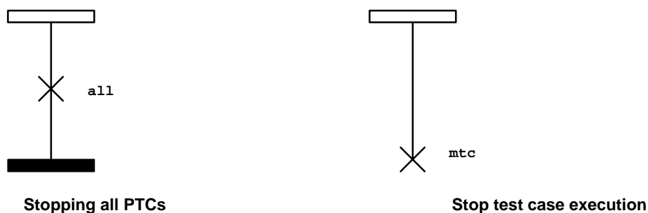
Figure 47: Special usages of the stop test component operation
