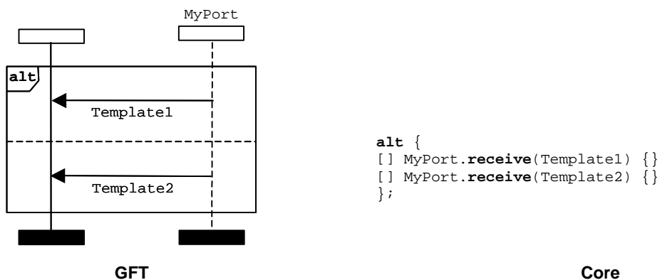
Figure 31: Alternative behaviour statement
