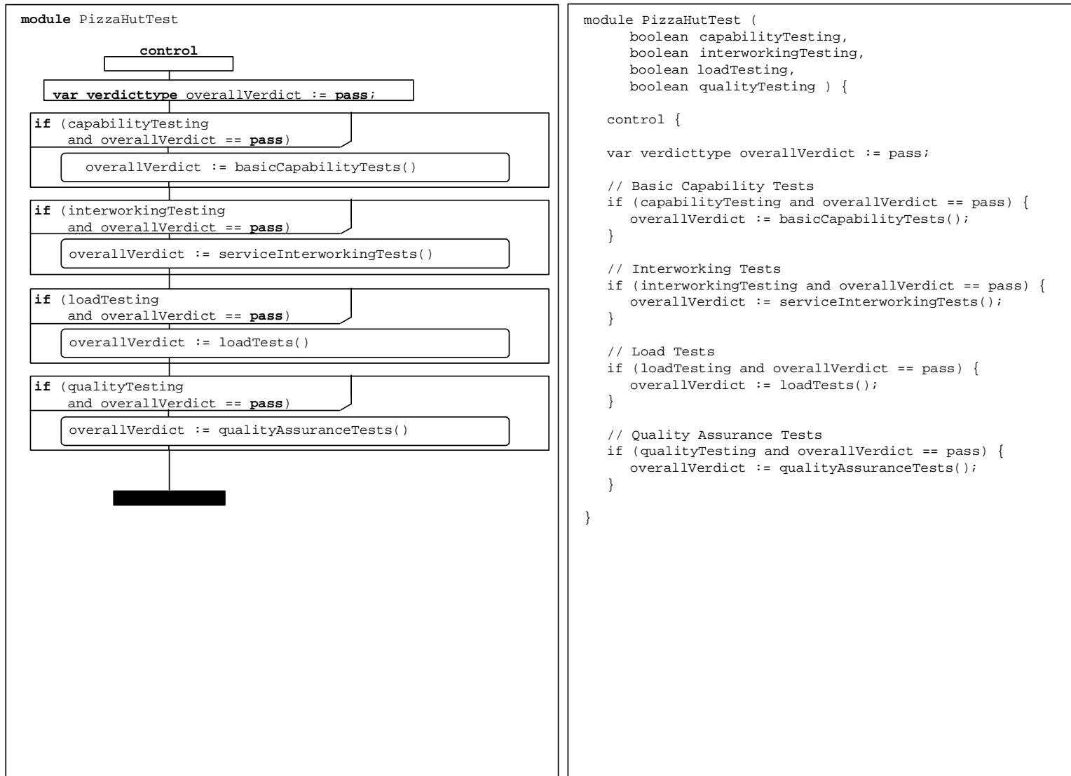
Figure E.9: Restaurant example - PizzaHutTest module
