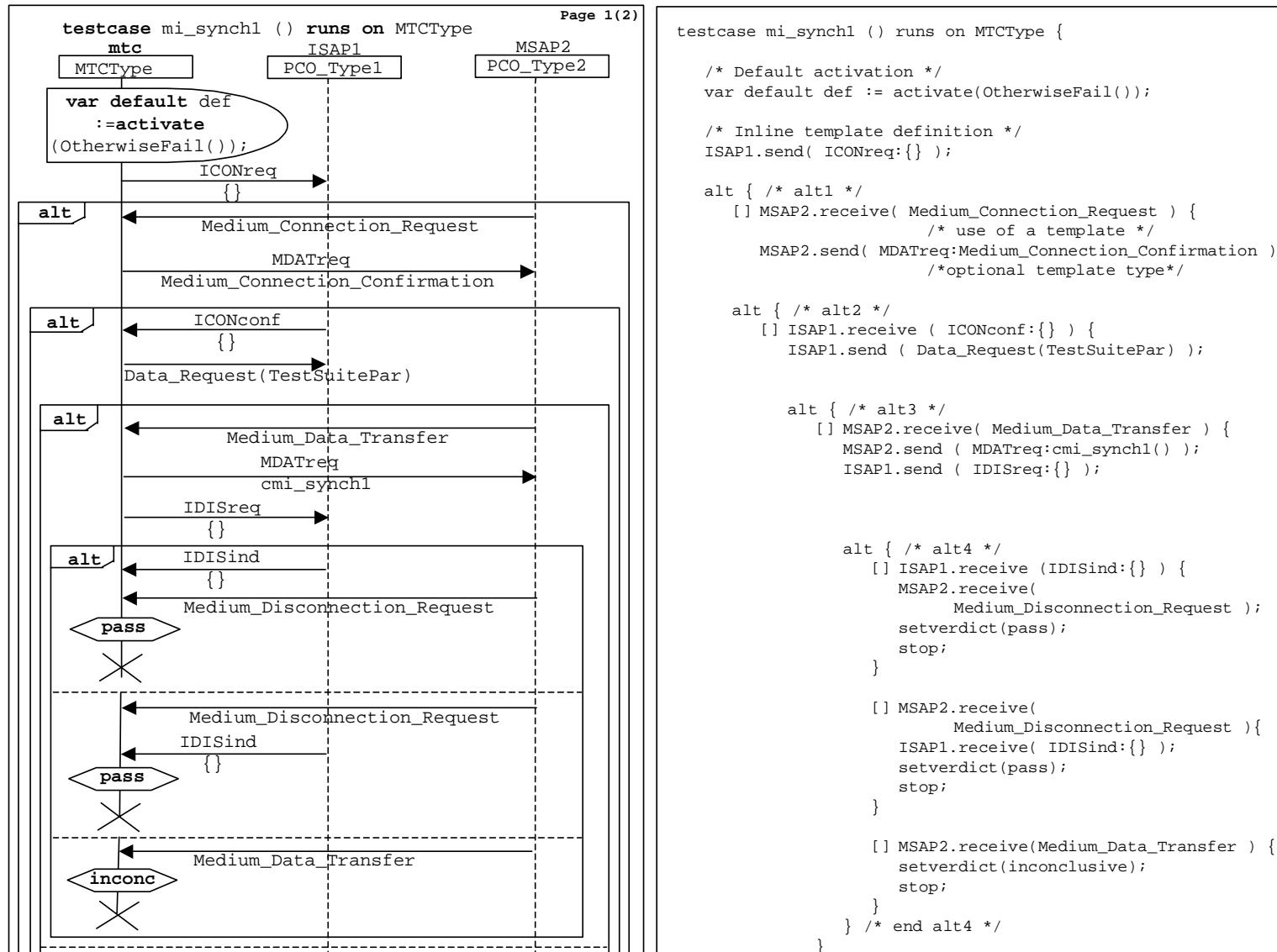
Figure E.10: INRES example - mi_synchl 1(2) test case
