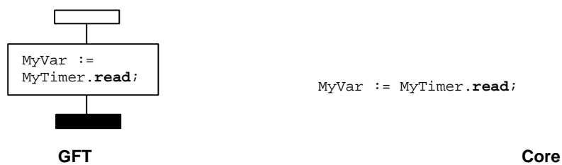
Figure 107: The read timer operation
