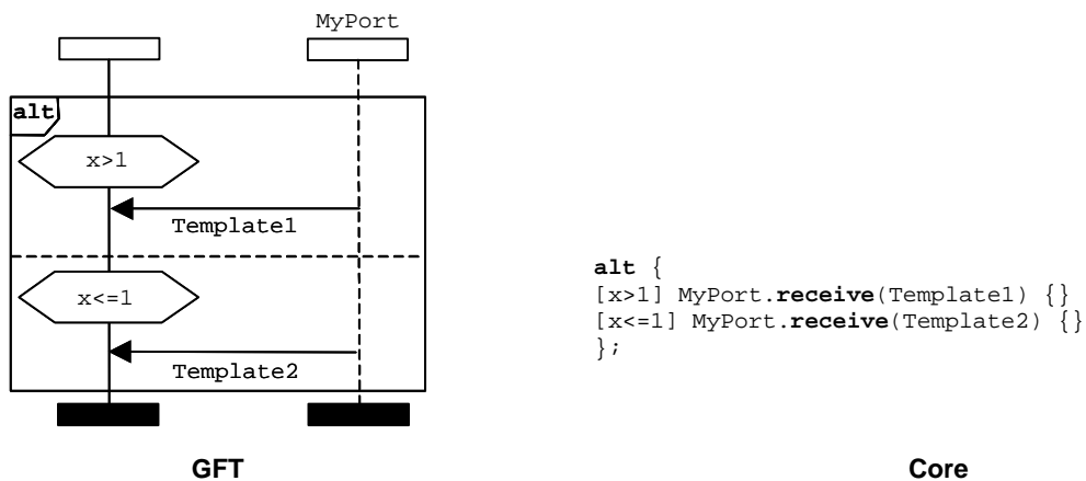
Figure 33: Selecting/deselecting an alternative
