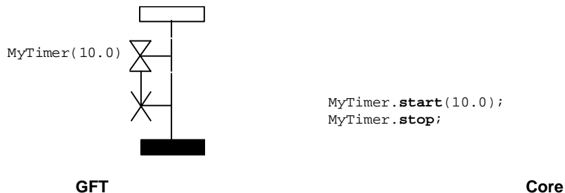
Figure 104: Connected start and stop timer symbols
