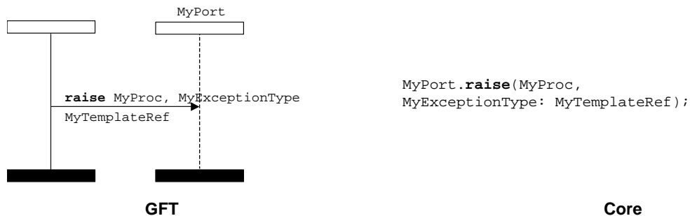
Figure 82: Raise operation with template reference
