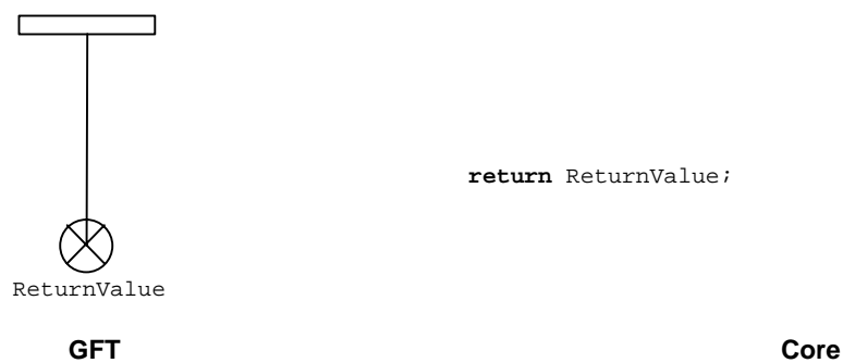
Figure 38: Return symbol with a return value
