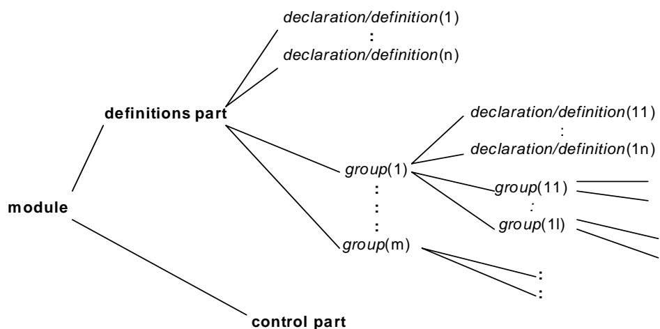
Figure 6: Structure of TTCN-3 modules
