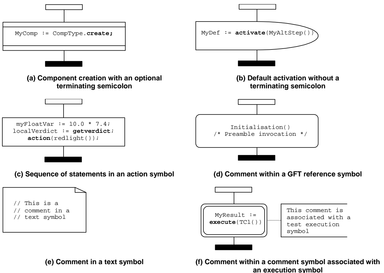
Figure 14: Examples for the effects of the general drawing rules
