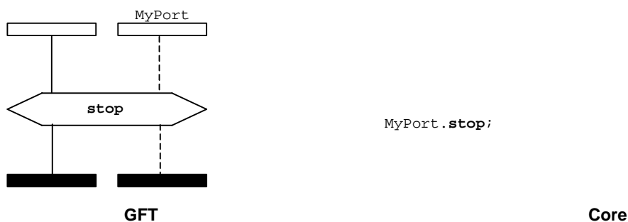
Figure 100: Stop port operation
