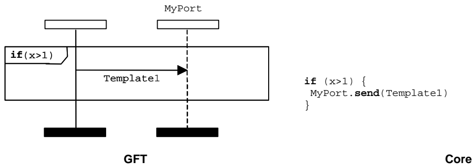
Figure 24: If-statement
