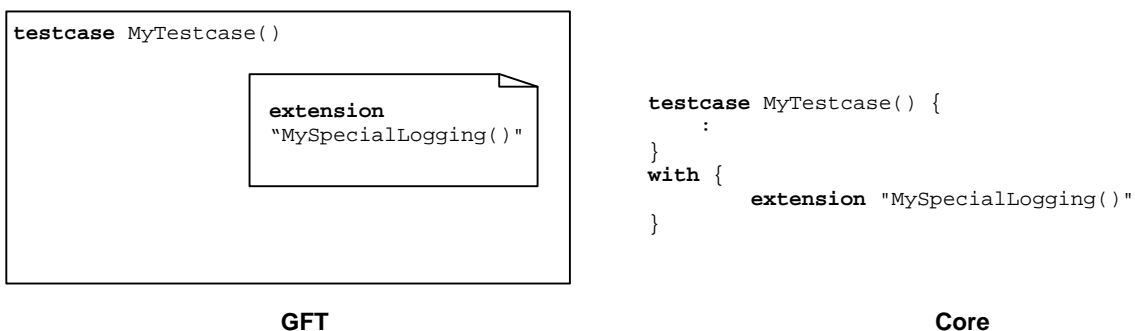
Figure 112: Specifying attributes
