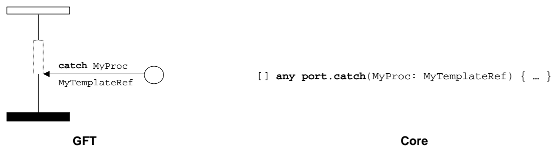
Figure 91: Catch on any port (within a call symbol)
