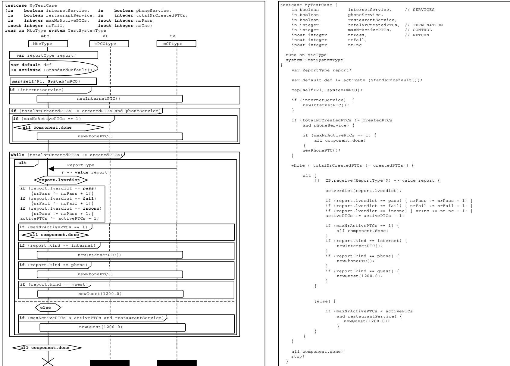
Figure E.1: Restaurant example - MyTestCase test case
