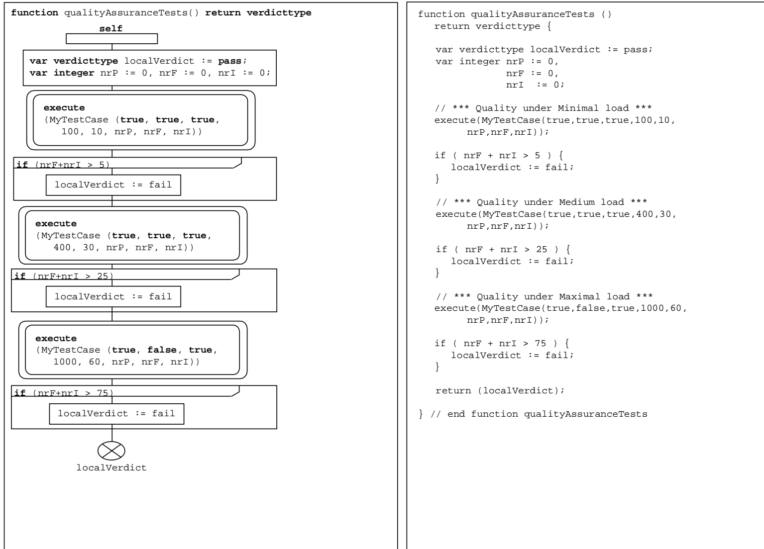
Figure E.8: Restaurant example - qualityAssuranceTests function
