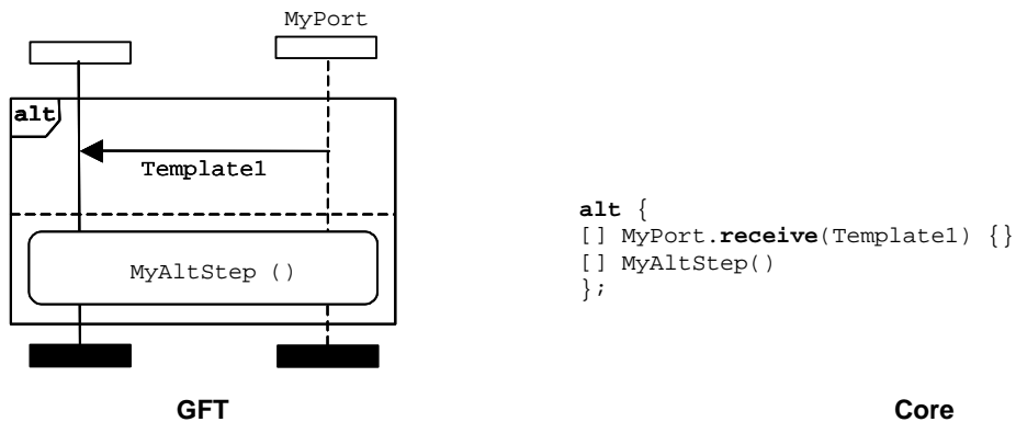
Figure 32: Alternative behaviour with altstep invocation
