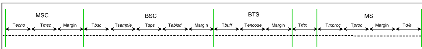
Figure 14.1: Reference Downlink delay distribution
