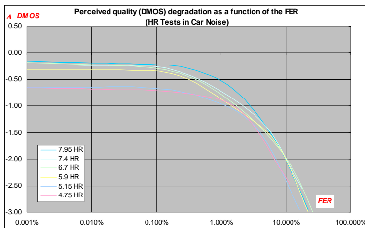
Figure D2b: Quality Degradation function of FER (HR Test Results)
