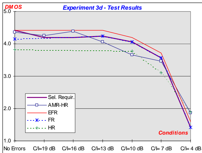
Figure 6.4: AMR performance curves for Experiment 3d (Half rate with Street Noise)
