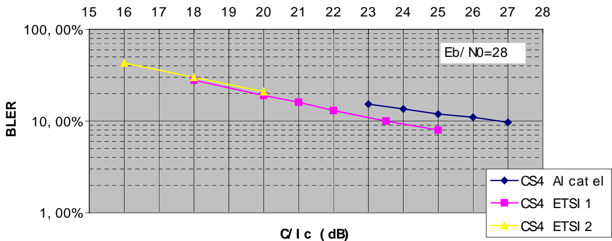
Figure 2 : TU50 no FH interference simulations (var. C/I_c ) - 1800 MHz
