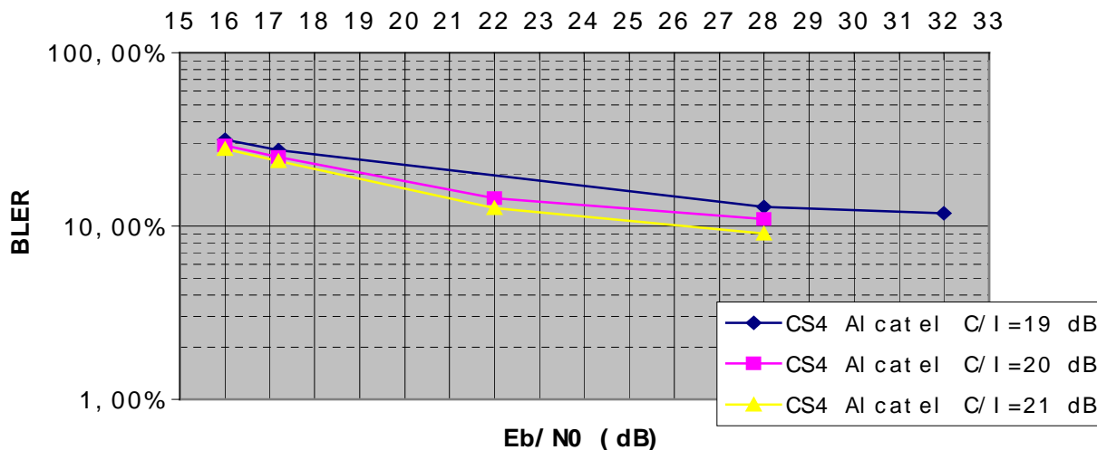
Figure 6 : TU 3 no FH interference simulations (var. Eb/N0) - 900 MHz
