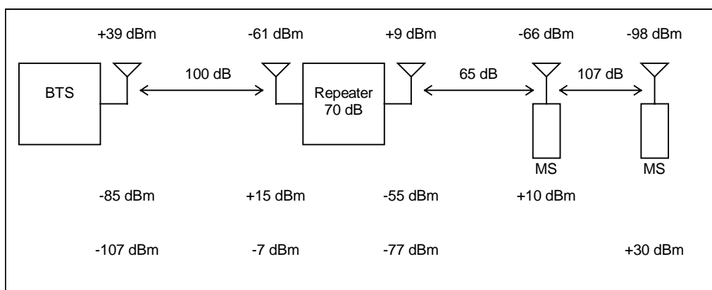
Figure 3 Outdoor Repeater Scenario
