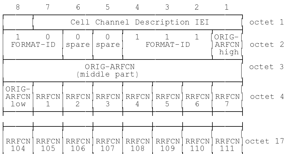
Figure 10.15/GSM 04.08
