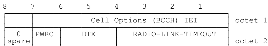
Figure 10.17/GSM 04.08: Cell Options (BCCH) information element
