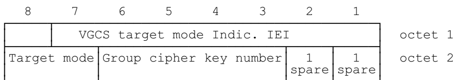
Figure 10.44f/GSM 04.08: VGCS target mode Indication information element
