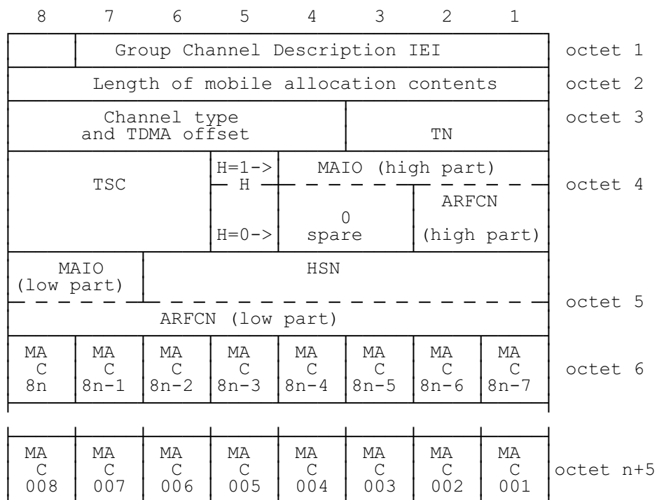
Figure 10.44i/GSM 04.08: Group Channel Description information element
