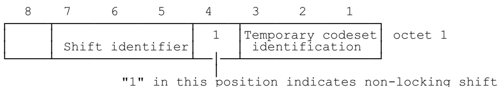
Figure 10.69/GSM 04.08: Non-locking shift element
