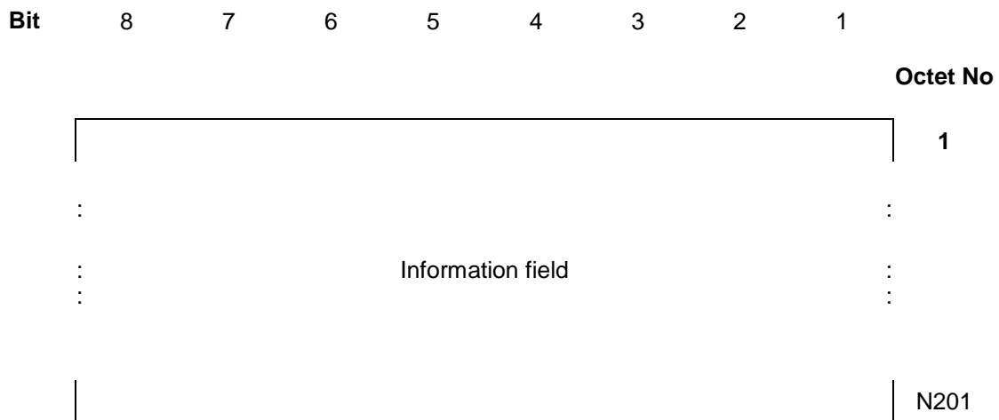
Figure 1/GSM 04.06 (sheet 2 of 3): General frame formats
