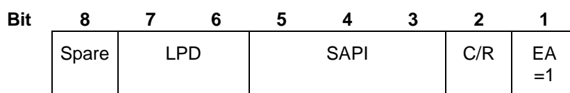
Figure 4/GSM 04.06: Address field format
