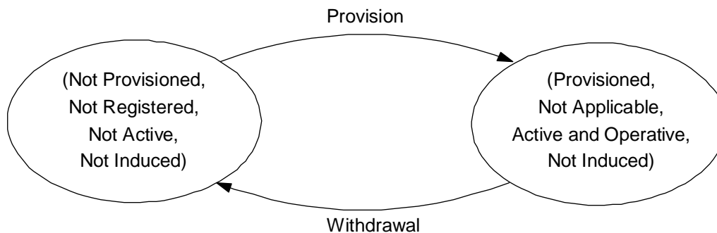
Figure 2.4: State transition model for AoCC
