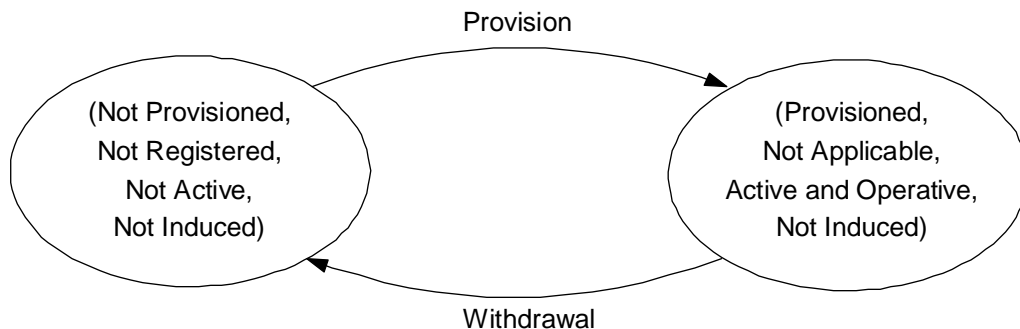
Figure 1.4: State transition model for AoCI
