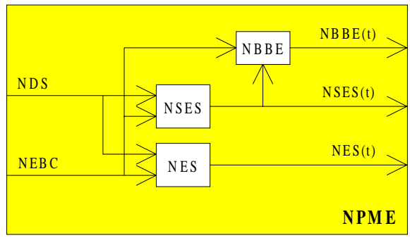
Figure 20: Near-end performance monitoring event (NPME) function
