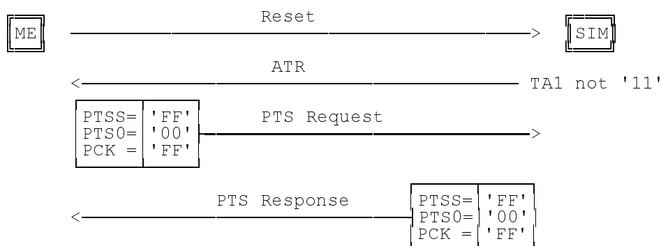
Figure 1: PTS procedure
