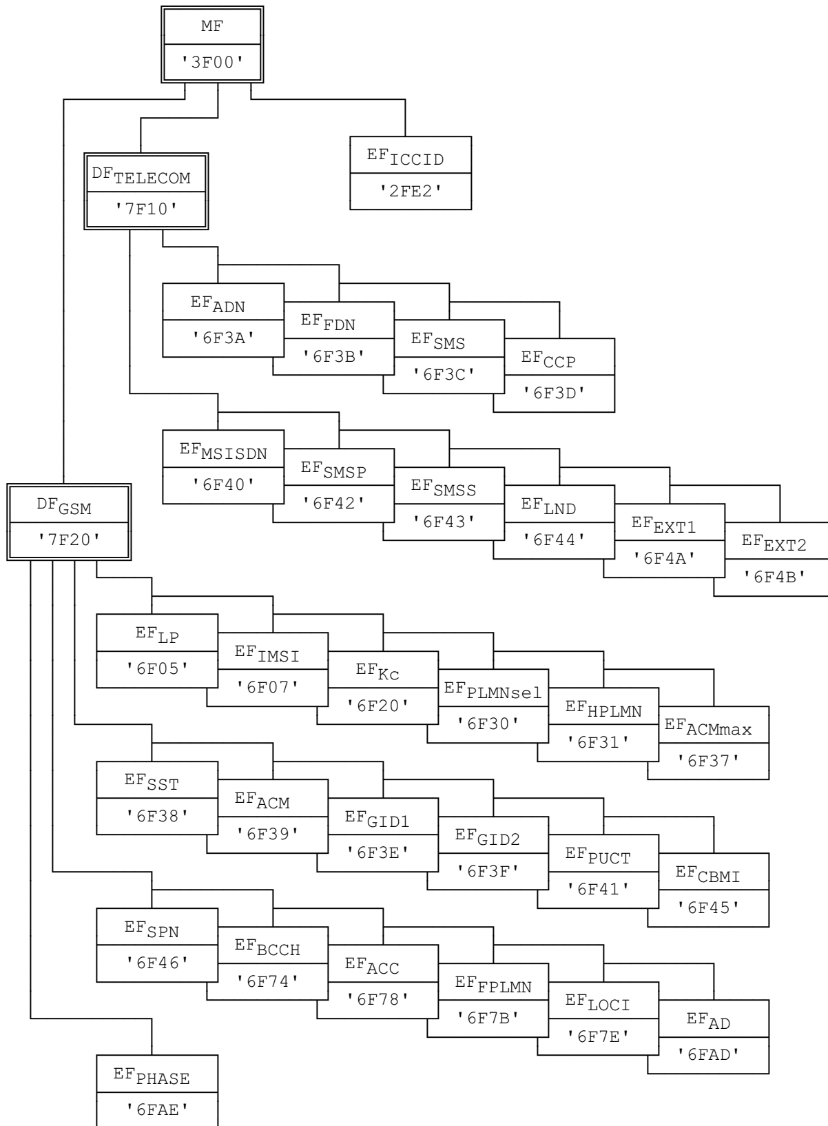
Figure 7: File identifiers and directory structures of GSM
