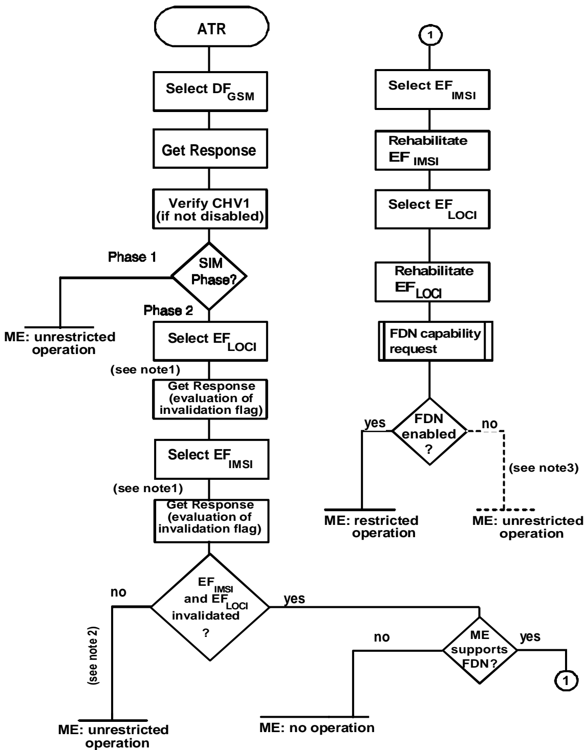
Example of an Initialisation Procedure of a FDN SIM (see 11.2.1)
