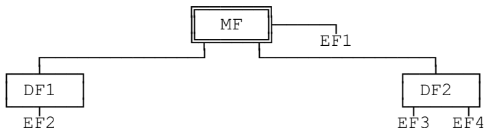
Figure 6: Logical structure
