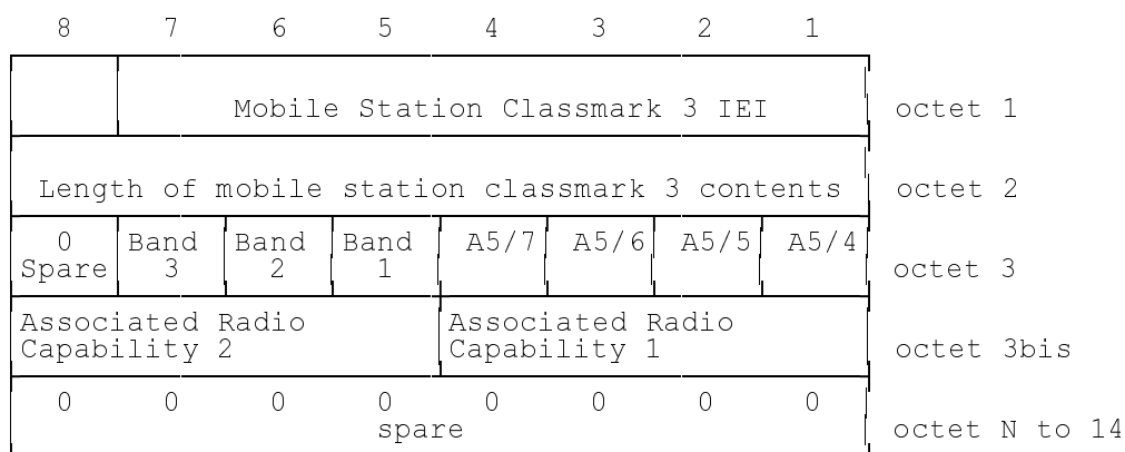
FIGURE 10.8/GSM 04.08 Mobile Station Classmark 3 information element
