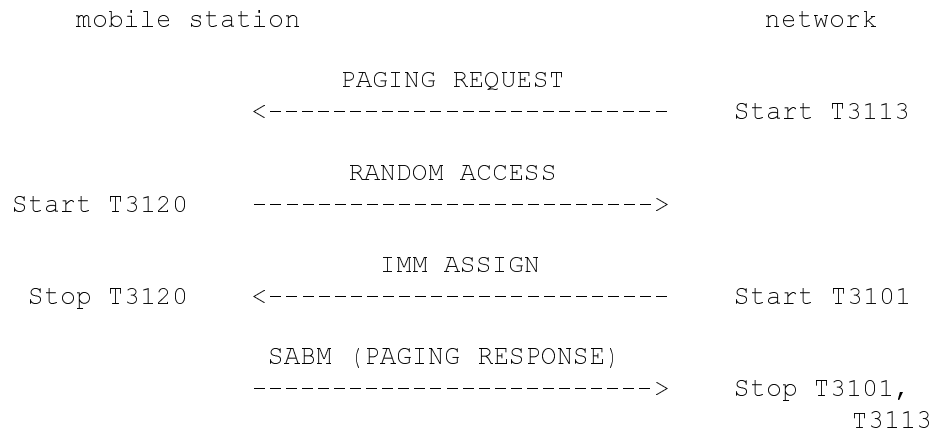
Figure 3.2/GSM 04.08 Paging sequence
