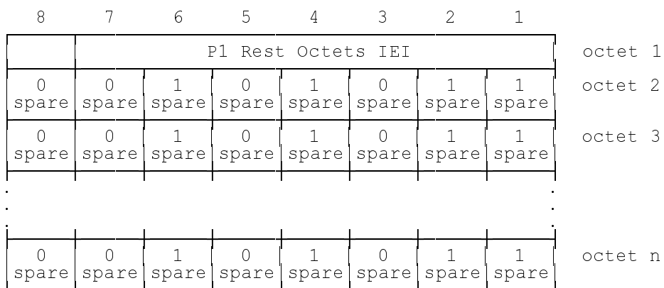
FIGURE 10.41/GSM 04.08 P1 Rest Octets information element
