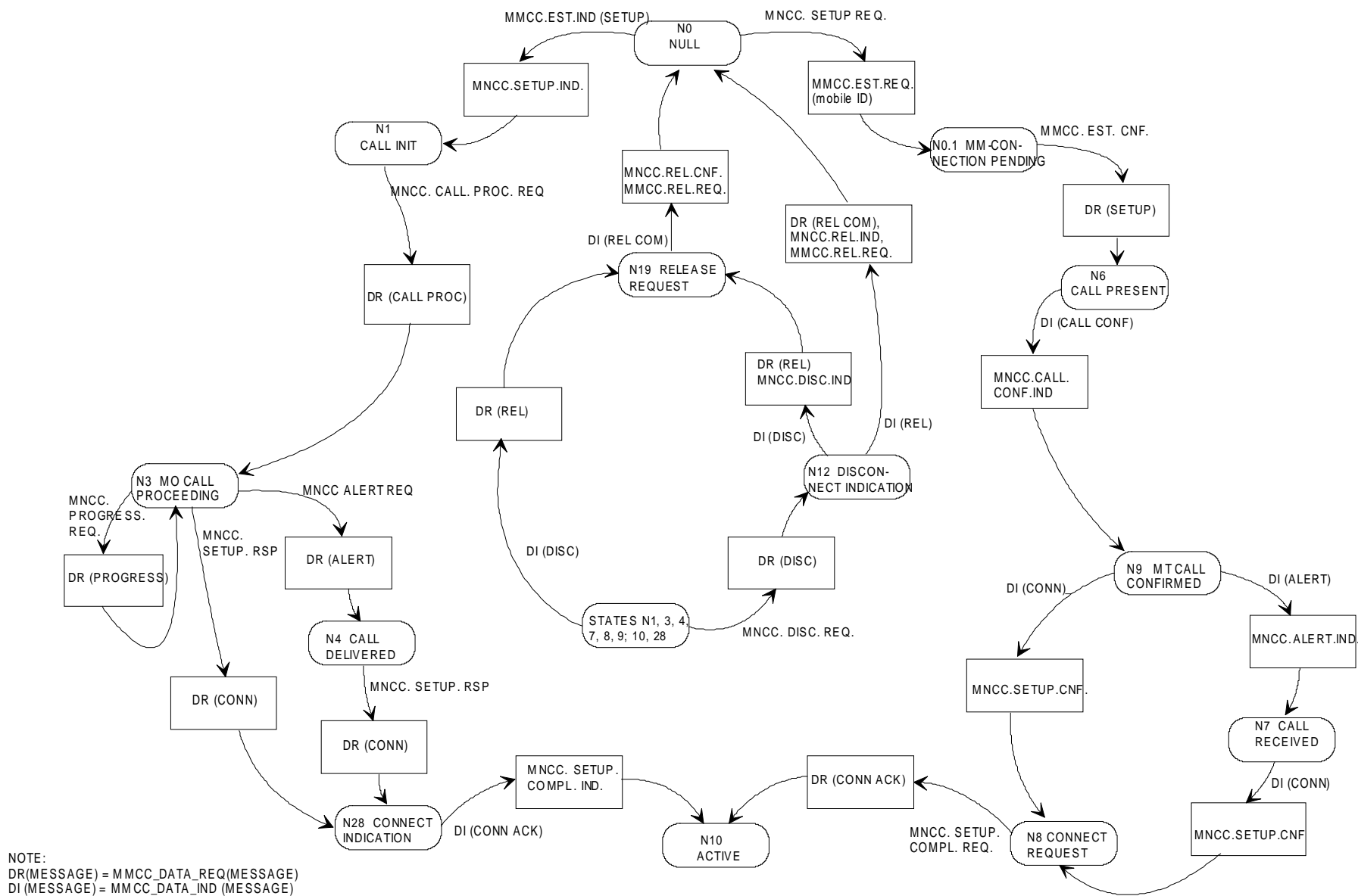
FIGURE 5.1b/GSM 04.08 Overview call control protocol/Network side
