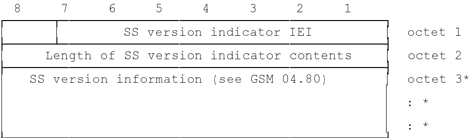
Figure 10.91/GSM 04.08
