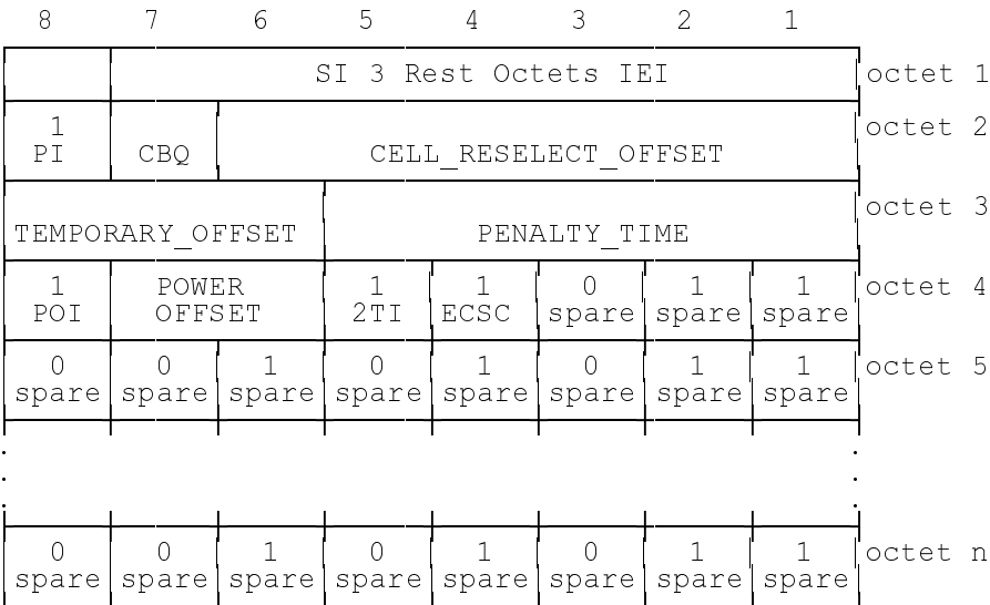
FIGURE 10.52h/GSM 04.08 SI 3 Rest Octets information element for PI=H & POI=H & 2TI=H & ECSC=L
