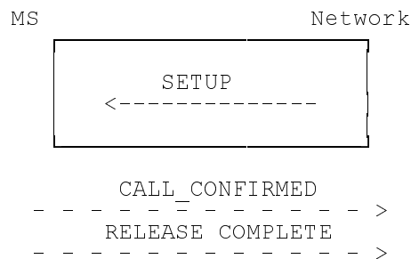
Figure 5.6/GSM 04.08 Mobile terminating call initiation and possible subsequent responses.
