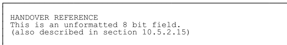
FIGURE 9.2/GSM 04.08 HANDOVER ACCESS message content
