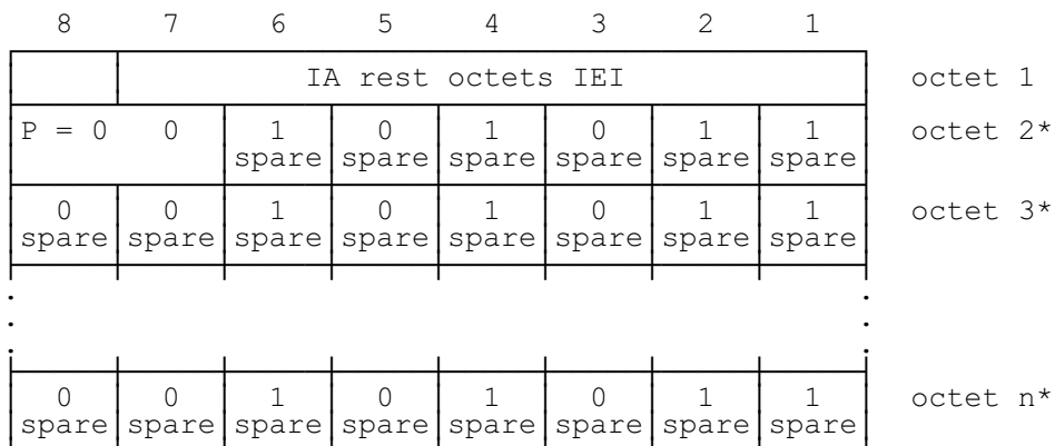
FIGURE 10.34/GSM 04.08 IA rest octets information element, P=00
