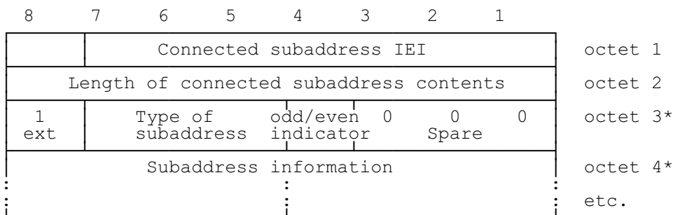
Figure 10.81/GSM 04.08
