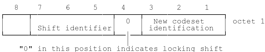
Figure 10.68/GSM 04.08: Locking shift element
