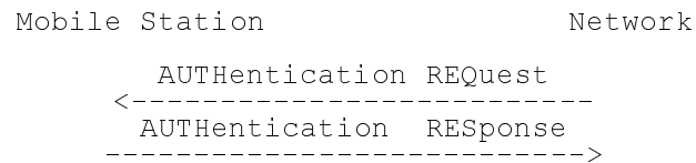
Figure 7.5/GSM 04.08: Authentication
