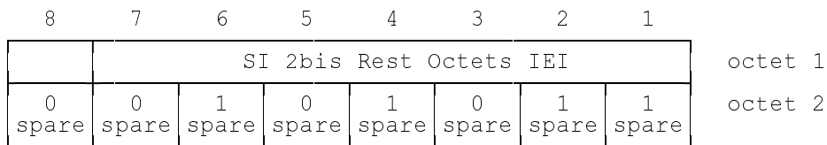
Figure 10.51/GSM 04.08: SI 2bis Rest Octets information element
