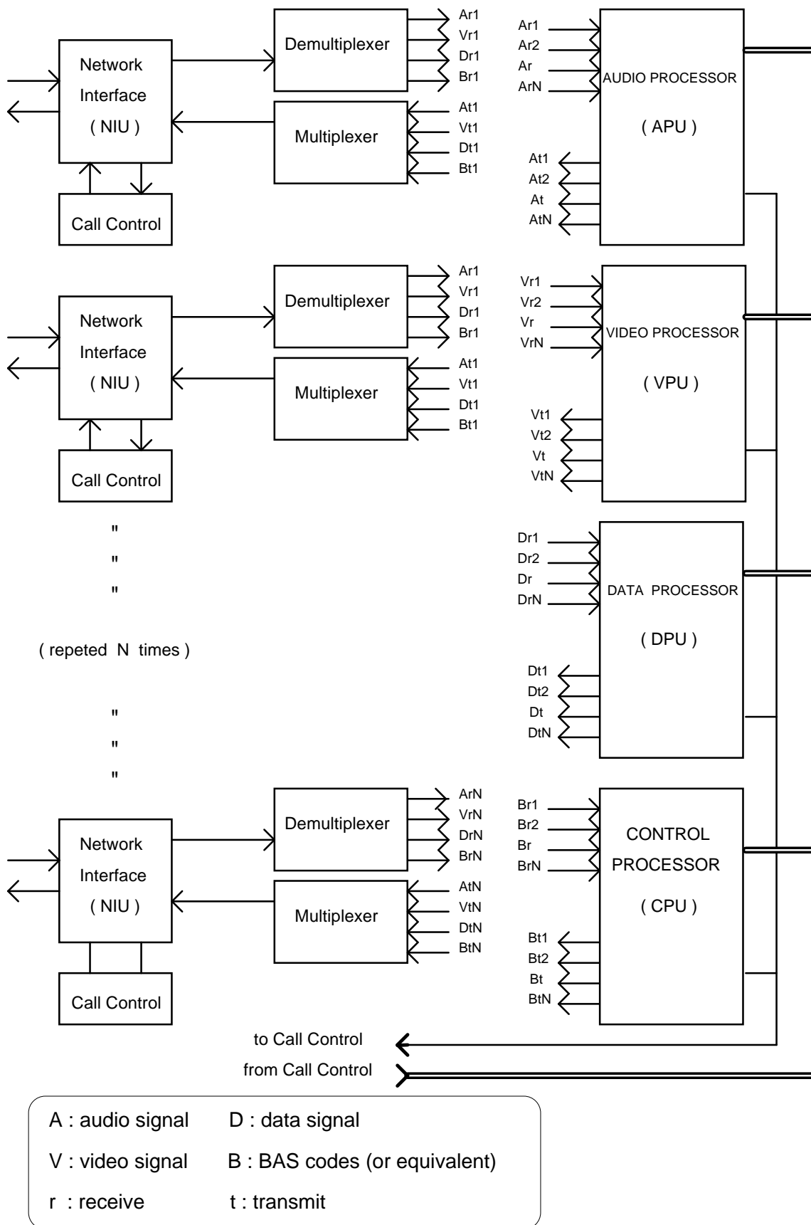
Figure 1: Schematic of a Multipoint Control Unit
