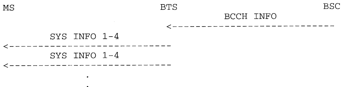
Figure 7-25: Broadcast information modify - normal case -----
