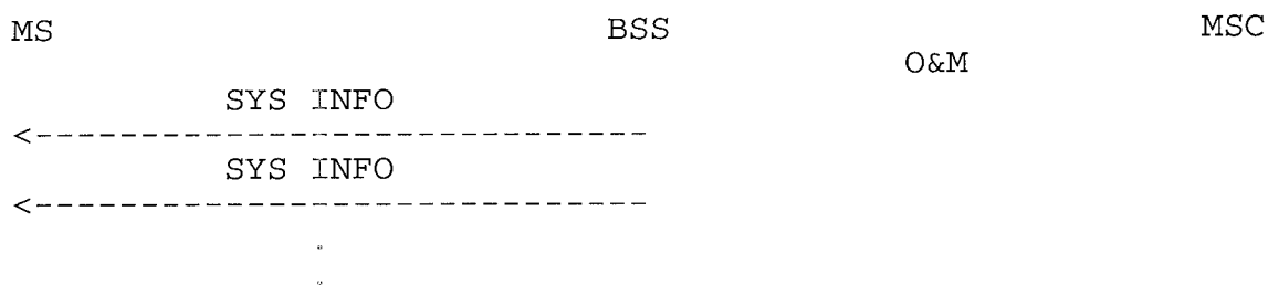
Figure 5-1: System information - normal case
