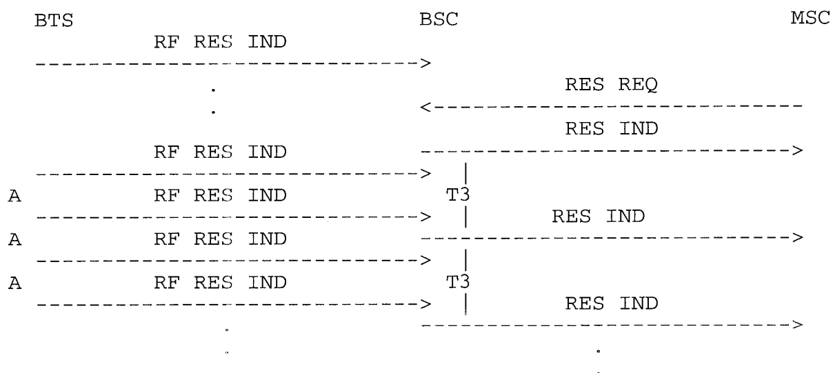
Figure 6-28: Radio resource indication - normal case
