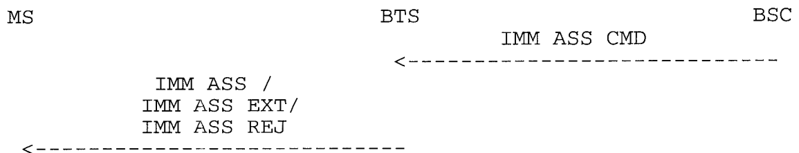
Figure 7-26: Immediate assignment - normal case -----
