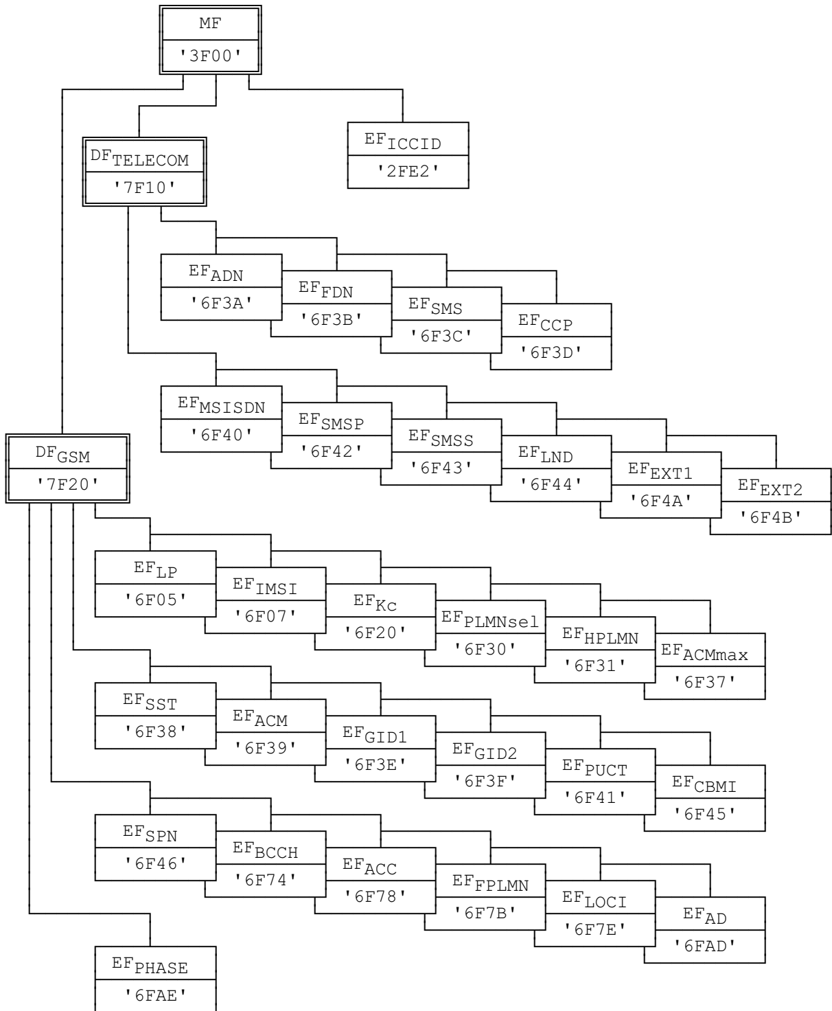
Figure 8: File identifiers and directory structures of GSM
